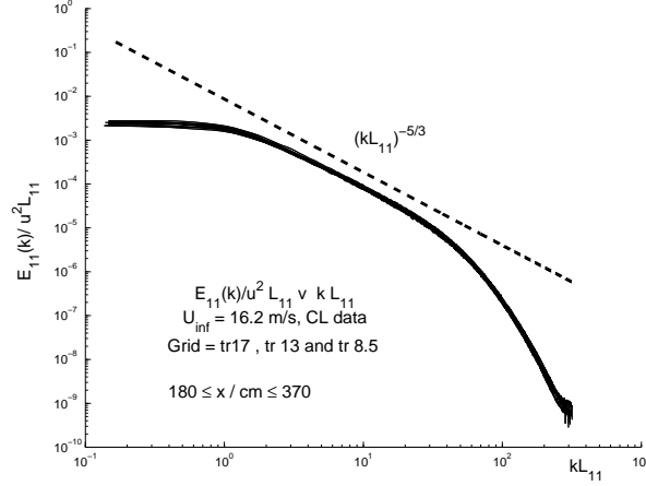
FIG. 14: E_{11}(k)/(u'^2 L_u) as a function of k_1 L_u for all three grids at one of our highest values of U_\infty , U_\infty \approx 16m/s , and at the following values of x all larger than x_{peak} : x = 1.8m, 2.1m, 2.8m, 3.0m, 3.2m and 3.7m for t_r = 17 where x_{peak} \approx 1.2m ; x = 2.8m, 3.0m, 3.2m and 3.7m for t_r = 13 where x_{peak} \approx 1.45m ; x = 3.2m and 3.7m for t_r = 8.5 where x_{peak} \approx 1.8m .
