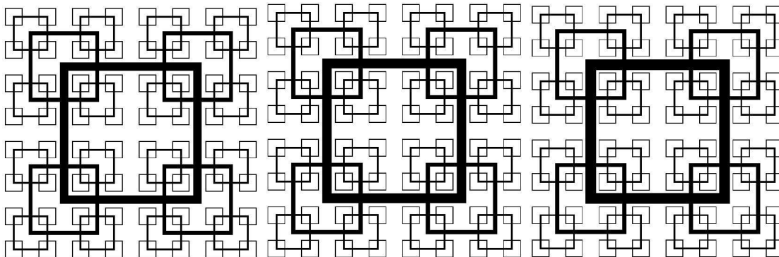
FIG. 1: Scaled diagrams of space-filling square grids for the T = 0.46m tunnel: t_r = 8.5, 13.0, 17.0
