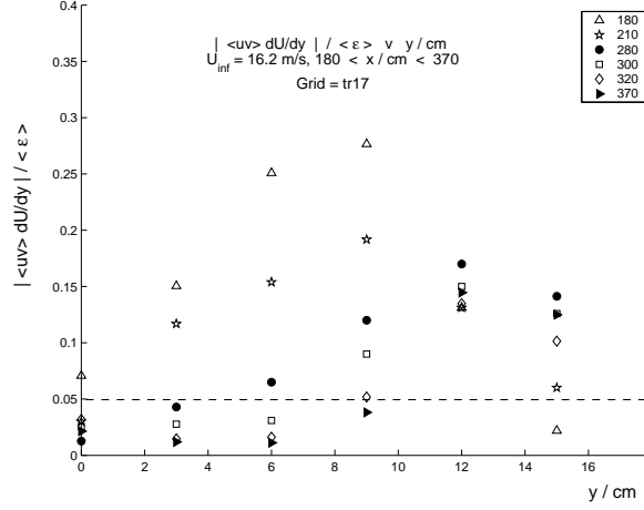
FIG. 6: Turbulence production rate by \frac{\partial U}{\partial y} normalised by the local dissipation rate \epsilon at various streamwise locations between x = 180\text{cm} and x = 370\text{cm} and various cross-stream locations between y = 0\text{cm} and y = 18\text{cm} downstream from the t_r = 17.0 grid ( x_{peak} \approx 1.2\text{m} ) for U_\infty = 16.2\text{m/s} . We plot |\langle uv \rangle \frac{\partial U}{\partial y}| as a function of y (in \text{cm} ) for various values of x (in \text{cm} in the insert).
