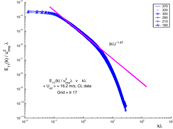
FIG. 13: E_{11}(k_1)/(u'^2 \lambda) as a function of k_1 \lambda for the t_r = 17 grid at one of our highest values of U_\infty , U_\infty = 16m/s , and at different values of x between x_{peak} and 3x_{peak} . The insert gives the values of x in cm corresponding to each spectral curve.
