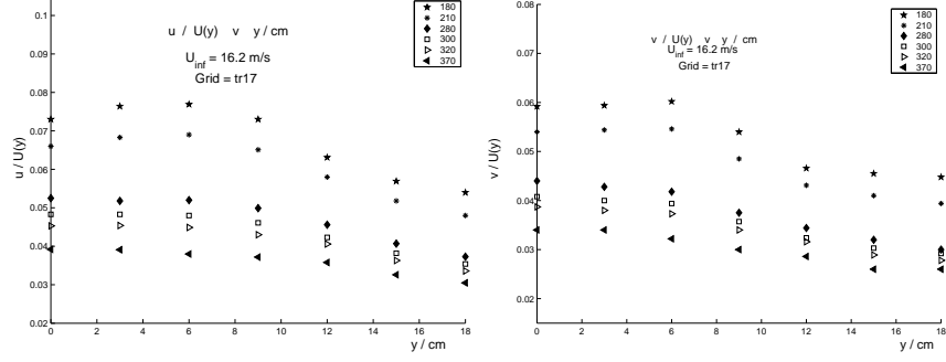
FIG. 4: Profiles of rms turbulence velocities at various streamwise locations between x = 180\text{cm} and = 370\text{cm} (given in \text{cm} in the inserts) downstream from the t_r = 17.0 grid ( x_{peak} \approx 1.2\text{m} ) for U_\infty = 16.2\text{m/s} .
