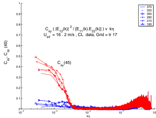
FIG. 7: Coherence spectra of u and v and (marked 45) of (u+v)/\sqrt{2} and (u-v)/\sqrt{2} at various centerline streamwise locations between x = 180\text{cm} and x = 370\text{cm} downstream from the t_r = 17.0 grid for U_\infty = 16.2\text{m/s} . ( \eta is the Kolmogorov length-scale.) The insert gives the values of x in \text{cm} corresponding to each coherence curve.
