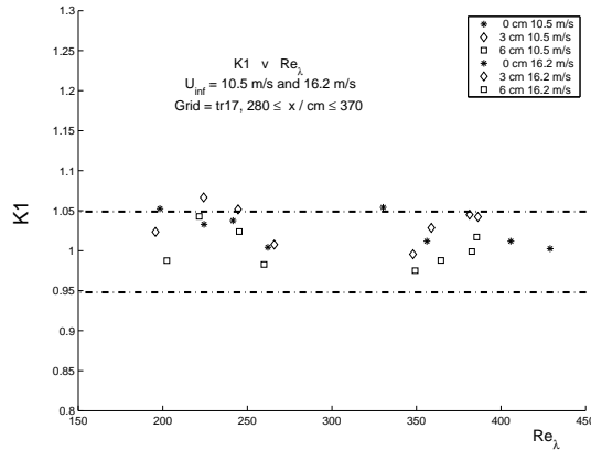
FIG. 8: Derivative ratio K_1 \equiv 2 \langle (\frac{\partial u}{\partial x})^2 \rangle / \langle (\frac{\partial v}{\partial x})^2 \rangle plotted as a function of local Reynolds number Re_\lambda at locations (x, y) downstream from the t_r = 17 fractal grid such that x is larger than 2x_{peak} and y = 0, 3, 6cm . Here, K_1 is obtained after filtering out of wavenumbers k_1 \eta \gtrsim 10^{-1} , which are contaminated by cross-wire interactions, see figure 7. Typical values 23,24 of K_1 found in various regions of various turbulent flows where local isotropy may be expected to hold are scattered between about 0.9 and about 2.
