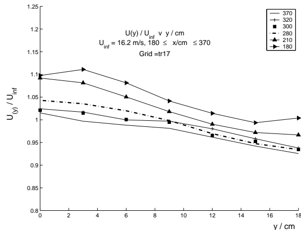
FIG. 3: Mean flow profiles at various streamwise locations between x = 180cm and x = 370cm (given in cm in the insert) downstream from the t_r = 17.0 grid ( x_{peak} \approx 1.2m ) for U_\infty = 16.2m/s . These profiles settle into a shape which varies little with x for x larger than about 2x_{peak} . In the region x \gtrsim 2x_{peak} and -10cm \leq y \leq 10cm (note that L_{max}/2 \approx 12cm ), these profiles are approximately homogeneous.
