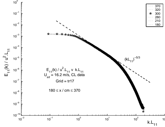
FIG. 12: E_{11}(k_1)/(u'^2 L_u) as a function of k_1 L_u for the t_r = 17 grid at one of our highest values of U_\infty , U_\infty = 16\text{m/s} , and at different values of x between x_{peak} and 3x_{peak} . The insert gives the values of x in cm corresponding to each spectral curve.
