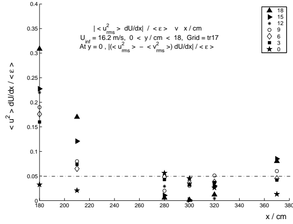
FIG. 5: Turbulence production rate by \frac{\partial U}{\partial x} normalised by the local dissipation rate \epsilon at various streamwise locations between x = 180\text{cm} and = 370\text{cm} and various cross-stream locations between y = 0\text{cm} and y = 18\text{cm} (in \text{cm} in the insert) downstream from the t_r = 17.0 grid ( x_{peak} \approx 1.2\text{m} ) for U_\infty = 16.2\text{m/s} . We plot u'^2 \frac{\partial U}{\partial x} as a function of x for various values of y \neq 0 . For y = 0 , we plot the modulus of (u'^2 - v'^2) \frac{\partial U}{\partial x} because of the grid symmetry with respect to a 90^\circ rotation about the centerline. The correction v'^2 \frac{\partial U}{\partial x} comes from incompressibility 22 which implies an effect of longitudinal mean velocity gradients in the y and/or z directions too.
