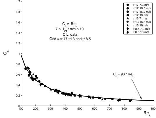
FIG. 10: C_\epsilon = \epsilon L_u / u'^3 as a function of Re_\lambda . Nine different cases are presented corresponding to nine different combinations of grid (value of t_r ) and U_\infty . For each case, measurements are reported from different streamwise centreline locations x in the decay region between x_{peak} and 3x_{peak} . The insert gives the grid and value of U_\infty corresponding to each set of data points.
