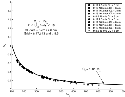
FIG. 11: C_\epsilon = \epsilon L_u / u'^3 as a function of Re_\lambda off centreline. Ten different cases are presented corresponding to ten different combinations of grid (value of t_r ), U_\infty and y = 3\text{cm} or 6\text{cm} . For each case, measurements are reported from different streamwise centreline locations x in the decay region between x_{peak} and 3x_{peak} . The insert gives the grid and values of U_\infty and y corresponding to each set of data points.
