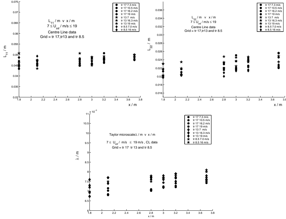
FIG. 2: The longitudinal and lateral integral length-scales L_u and L_v (in meters) and the Taylor microscale \lambda (which lies in the range 6.7mm to 8.0mm in all cases) as functions of x (in meters from the grid) on the centreline for the three different grids ( t_r = 17, 13, 8.5 ) and for different values of U_\infty . All points x are larger than x_{peak} which is approximately 1.2m, 1.45m and 1.8m for the grids t_r = 17, 13, 8.5 respectively. U_\infty is varied between 7m/s and 19m/s. The inserts give the grid and value of U_\infty corresponding to each data point.
