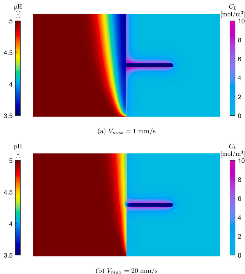
Fig. 12. Metal–electrolyte interactions: Effect of the electrolyte velocity on the pH and lattice hydrogen concentration at t = 5 min. The electrolyte velocity varies linearly from V_{max} at the left edge of the electrolyte, to 0 at the electrolyte–metal interface (see Fig. 7). Here, results are provided for the choices of (a) V_{max} = 1 mm/s and (b) V_{max} = 20 mm/s.
