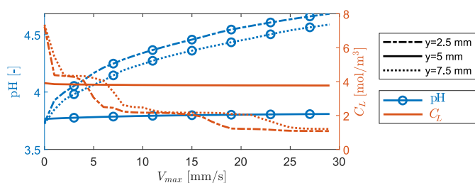
Fig. 13. Metal–electrolyte interactions: Effect of the electrolyte velocity on the pH (blue, left y-axis) and lattice hydrogen concentration (orange, right y-axis) at t = 5 min and various locations along the metal–electrolyte interface ( y , with y = 5 mm being the centre height).
