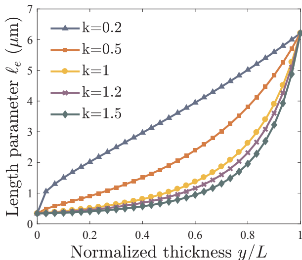
Fig. 1. Variation of the effective material length scale \ell_e along the material gradient direction.
