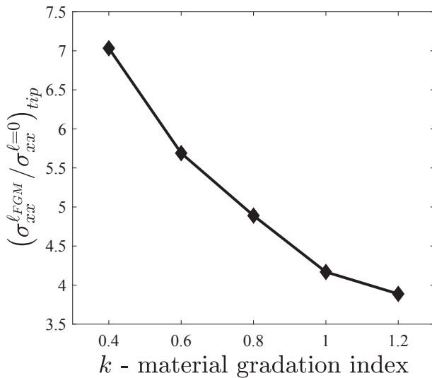
Fig. 13. Crack tip stress ratio as a function of the material gradient index k . Results are shown for the case of \ell_{FGM} and R_p = 0.0027 mm.
