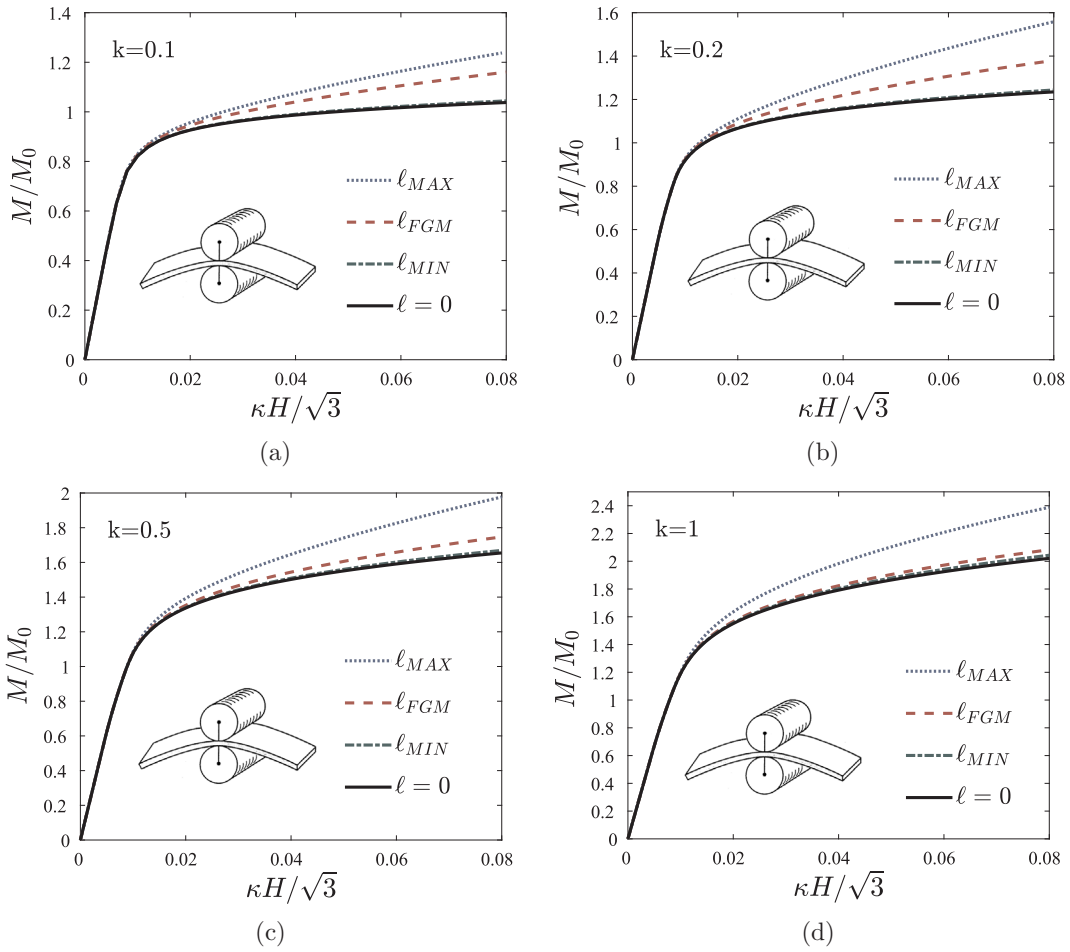
Fig. 3. Normalized moment versus curvature for conventional ( \ell = 0 ) and strain gradient plasticity theories. A functionally graded length parameter ( \ell_{FGM} ) has been considered, along with the limit cases of the stiffer ( \ell_{MAX} ) and the softer ( \ell_{MIN} ) compounds. Material gradient indexes: (a) k = 0.1 , (b) k = 0.2 , (c) k = 0.5 , and (d) k = 1 .
