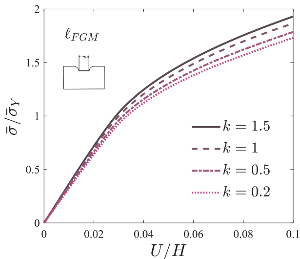
Fig. 8. Average non-dimensional indentation pressure as a function of non-dimensional indentation depth for different material gradient indexes in a functionally graded strain gradient solid.
