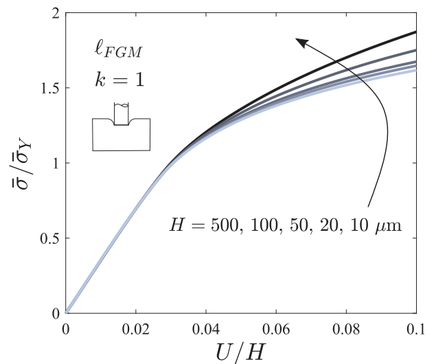
Fig. 9. Average non-dimensional indentation pressure as a function of non-dimensional indentation depth for different indenter sizes in a functionally graded strain gradient solid. The indentation depth is normalized by the reference indenter size: H = 20 \mu\text{m} .
