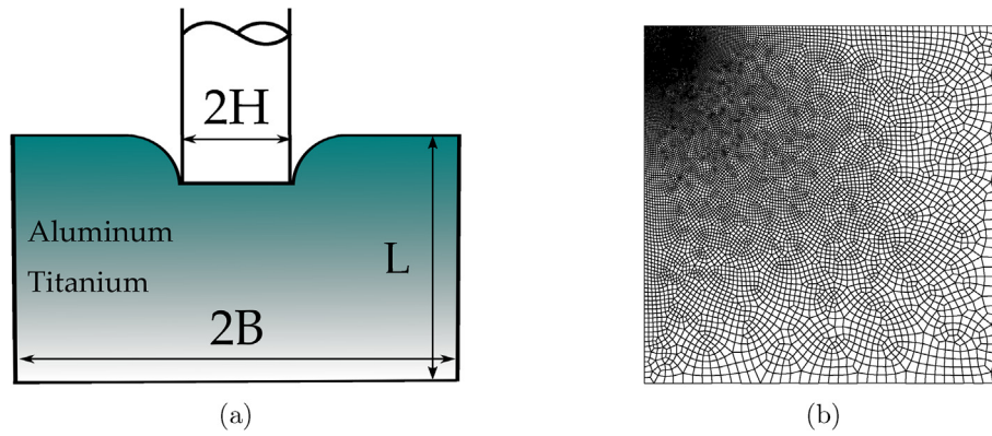
Fig. 6. Indentation in elasto-plastic FGMs: (a) geometry, and (b) finite element mesh.
