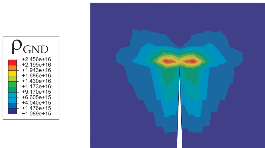
Fig. 12. Contour plot of the density of geometrically necessary dislocations in m^{-2} . Results are shown for the case of \ell_{MIN} and R_p = 0.00027 mm.
