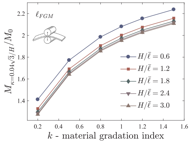
Fig. 5. Normalized bending moment in a functionally graded solid at a curvature \kappa = 0.04\sqrt{3}/H for different foil thicknesses and as a function of the material gradient index k .
