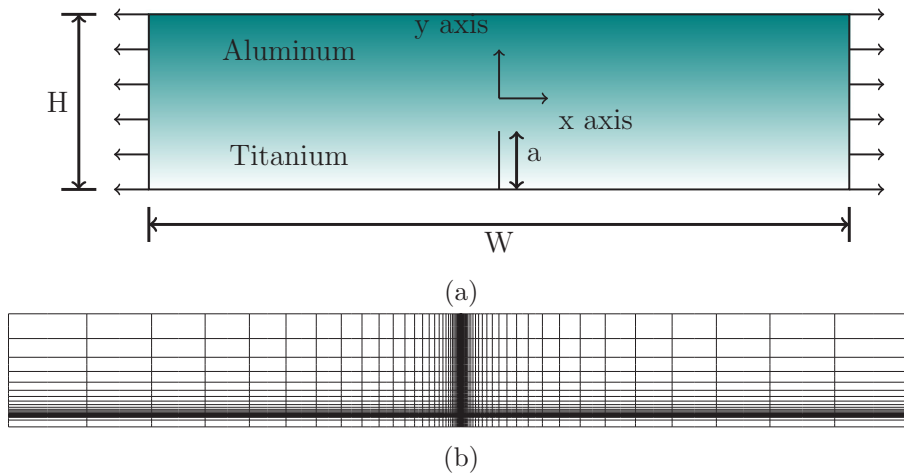
Fig. 10. Fracture analysis of a functionally graded plate: (a) Geometry and loading configuration and (b) finite element mesh.
