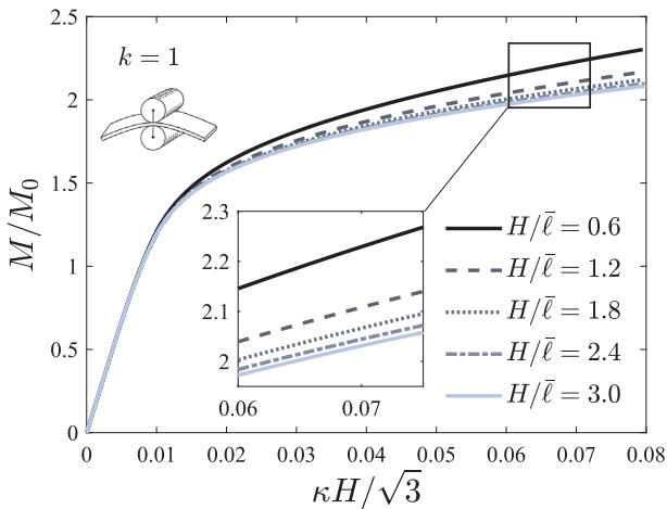
Fig. 4. Normalized moment versus curvature for different foil thicknesses in a functionally graded solid.
