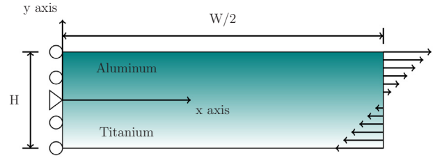
Fig. 2. Schematic representation of the numerical micro-bending experiments on thin metal-metal FGM films.
