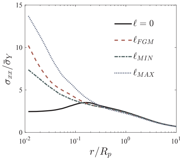
Fig. 11. Crack opening stress distribution in an FGM specimen for conventional ( \ell = 0 ) and strain gradient plasticity theories. A functionally graded length parameter ( \ell_{FGM} ) has been considered, along with the limit cases of the stiffer ( \ell_{MAX} ) and the softer ( \ell_{MIN} ) compounds. Material gradient index: k = 1 .
