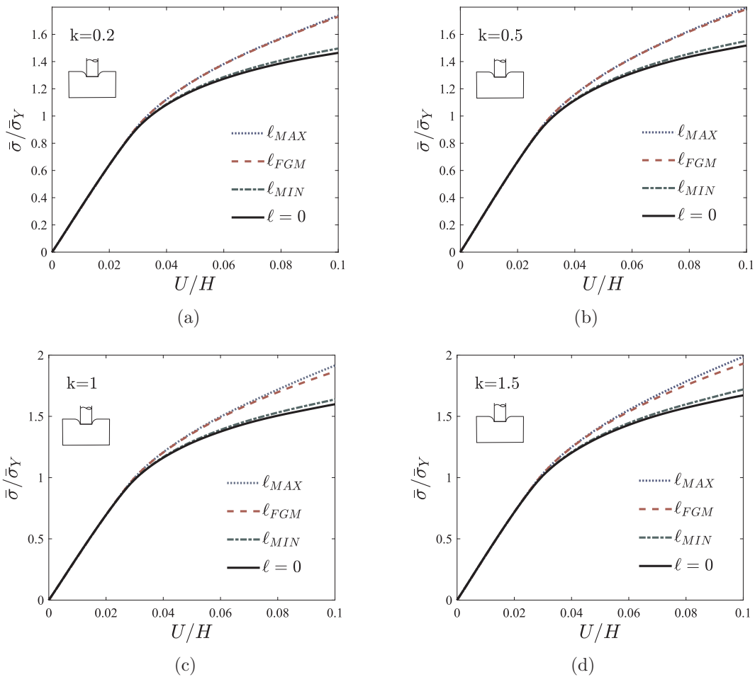
Fig. 7. Average non-dimensional indentation pressure as a function of non-dimensional indentation depth for conventional ( \ell = 0 ) and strain gradient plasticity theories. A functionally graded length parameter ( \ell_{FGM} ) has been considered, along with the limit cases of the stiffer ( \ell_{MAX} ) and the softer ( \ell_{MIN} ) compounds. Material gradient indexes: (a) k = 0.2 , (b) k = 0.5 , (c) k = 1 , and (d) k = 1.5 .
