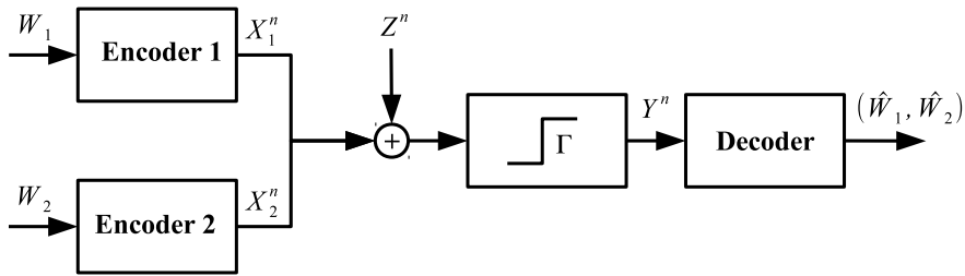
Figure 1: A two-transmitter Gaussian MAC with a one-bit ADC front end at the receiver.
