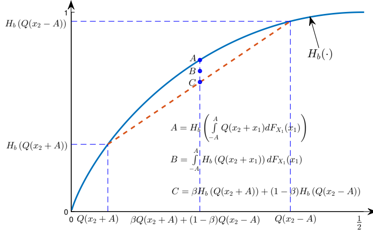
Figure H1: The figure depicting (98) and (100). Note that in the statement of Lemma 3, x_2 \rightarrow +\infty . Hence, we have assumed x_2 > A in the figure.
