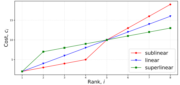
Fig. 2: Rank-cost dependencies.
