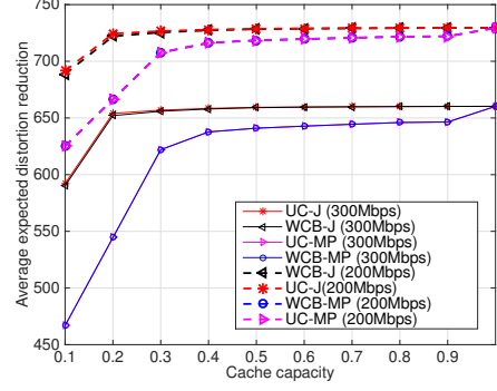
Fig. 2. Average expected distortion reduction vs the cache capacity.
