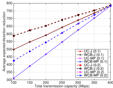
Fig. 3. Average expected distortion reduction vs the total transmission rate of the MBS.
