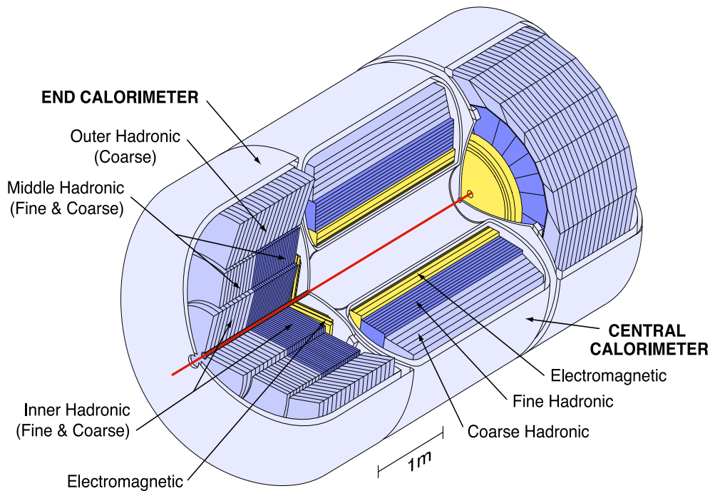
Figure 2.10: Three-dimensional view of the DØ calorimeter.
