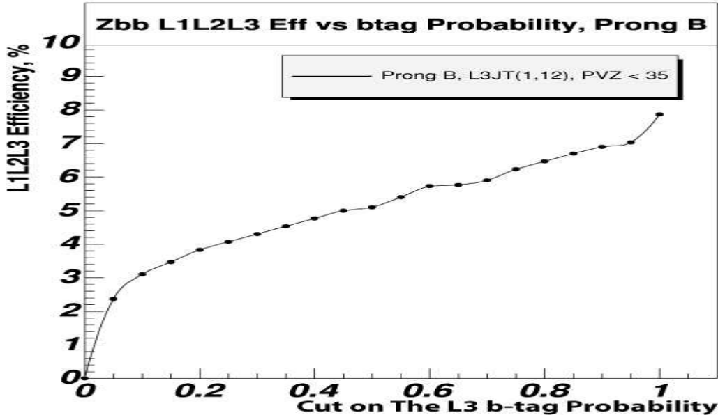
Figure 4.10: Signal efficiency as a function of L3 b -tag probability. The likelihood that the event is b -tagged increases as the probability tends to 0. Trigger combination applied here: one L2 jet above 6 GeV, one L3 jet above 12 GeV and an L3 primary vertex constraint of |z| < 35 cm.
