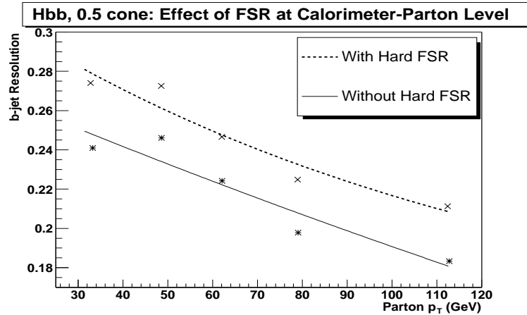
Figure 3.4: Effect of hard FSR on the b -jet resolution in ZH \rightarrow e^+e^-b\bar{b} at the calorimeter-parton level.
