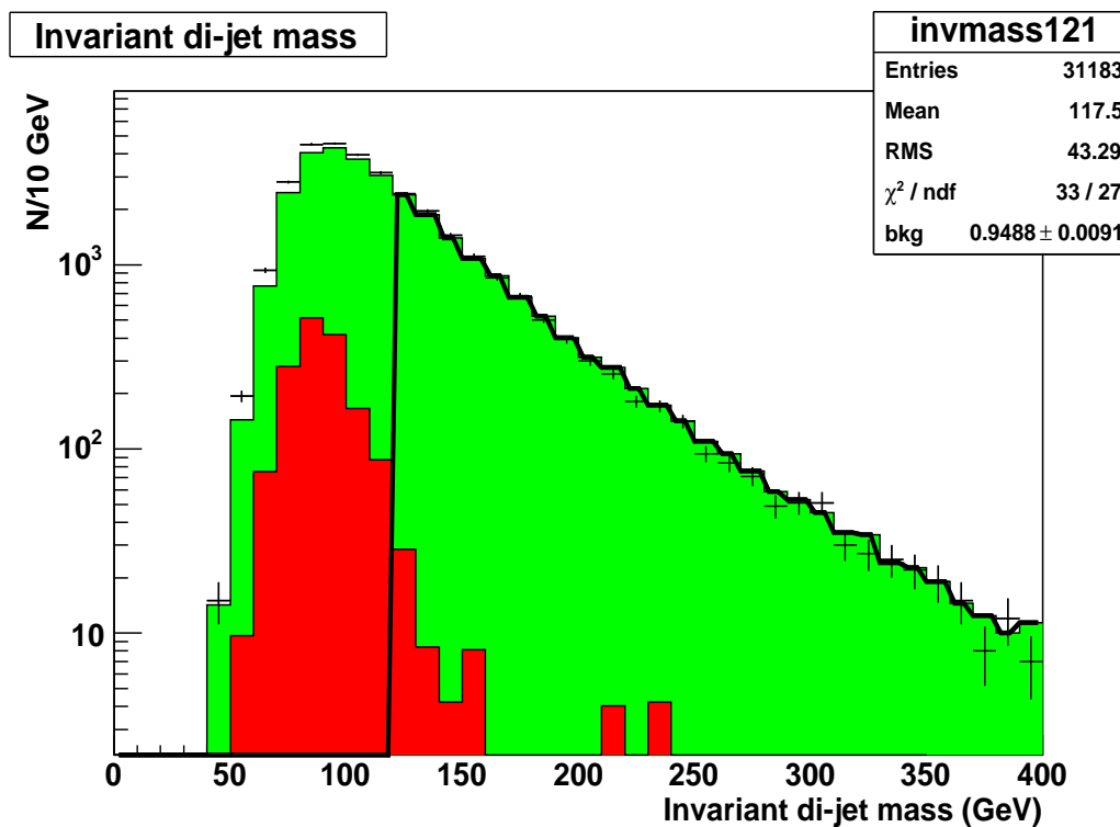
Figure 5.11: Invariant dijet mass in the pre-v13 data before background subtraction. Green (light grey) shaded histogram: expected background, estimated using a jet-based TRF from in-zone events and fitted with a one parameter fit to the observed data above 120 GeV/c 2 . Black points: total dijet mass distribution observed in data. Red (dark grey) shaded histogram: expected Z \rightarrow b\bar{b} signal from MC. The fit (bold black line) results in a correction to the background scale of 0.9488 \pm 0.0091 .
