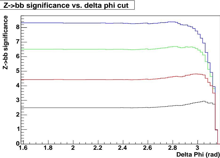
Figure 5.3: Effective signal significance as a function of \Delta\varphi cut in pre-v13 data, for a systematic error of 0% (blue (top line)), 0.5% (green (second line down)), 1% (red (third line down)) and 2% (black (bottom line)) on the number of background events. The dependence on \Delta\varphi is weak and a loose cut of 2.75 is applied to the pre-v13 analysis.
