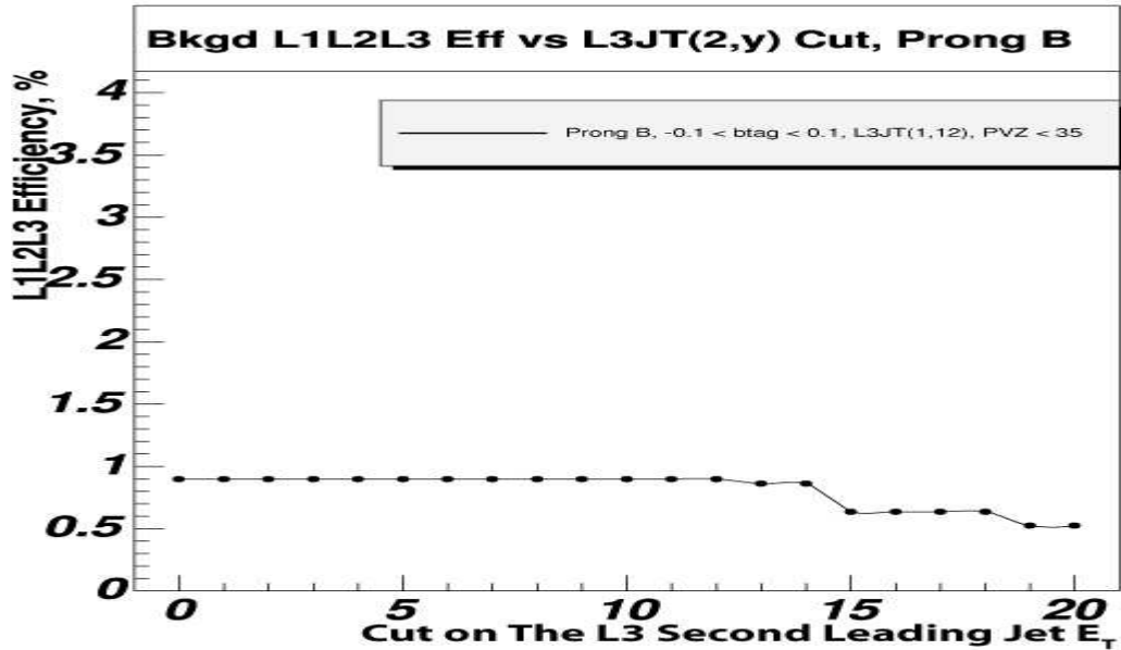
Figure 4.8: Background efficiency as a function of the cut on the second leading jet E_T at Level 3. Trigger combination applied while the cut on the L3 jet E_T was varied: one L2 jet above 6 GeV, one L3 jet above 12 GeV, an L3 b -tag probability < 0.1 and an L3 primary vertex constraint of |z| < 35 cm.
