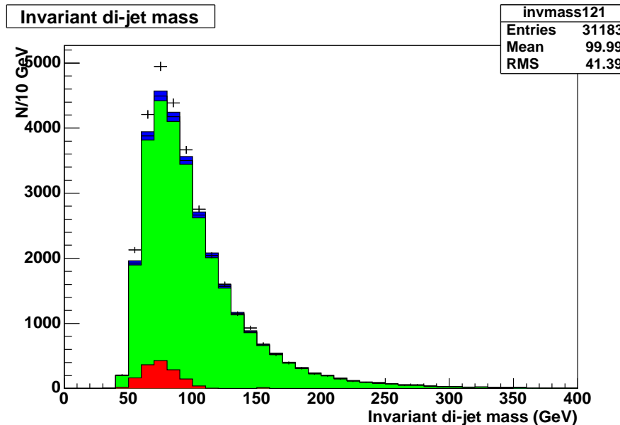
Figure B.7: Invariant dijet mass in the pre-v13 data before background subtraction. Green (light grey) shaded histogram: expected background, estimated using a jet-based TRF from in-zone events. The dark blue (black) band represents the \pm 1.2\% systematic error on the background from the normalisation fit. Black points: total dijet mass distribution observed in data. Red (dark grey) histogram: expected Z \rightarrow b\bar{b} signal from MC.
