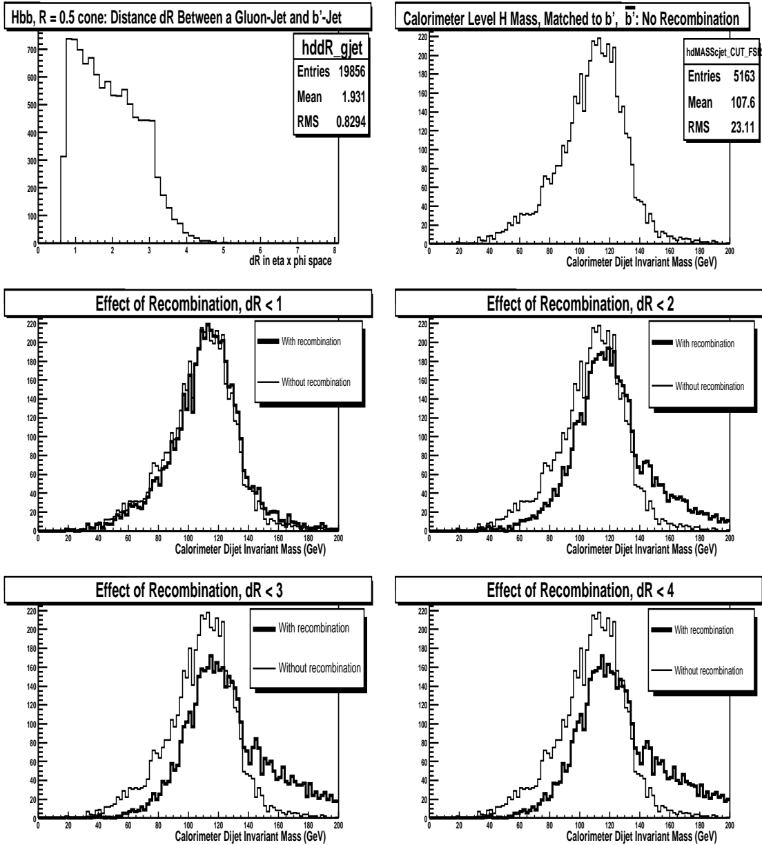
Figure 3.12: The effect of recombination on Higgs mass resolution. Top left: dR(b' -jet, gluon jet) distribution; top right: calorimeter dijet mass without recombination; the other plots show the effect of recombination for dR < 1, 2, 3, 4 .
