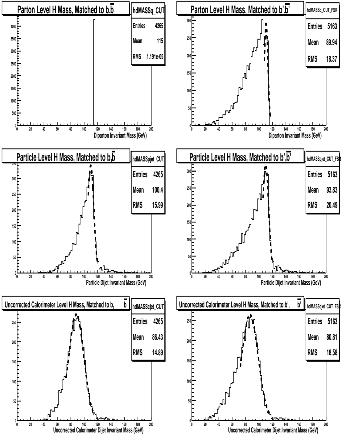
Figure 3.8: Reconstructed Higgs mass at parton (top), particle-jet (middle) and uncorrected calorimeter-jet (bottom) levels. Without hard FSR (left); with hard FSR (right). All jets are 0.5 cone. Dashed profiles show Gaussian fits to the central symmetric portion of the peak of each distribution (i.e. excluding any tails).
