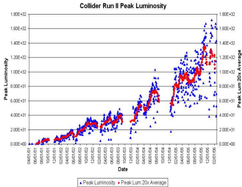
Figure 2.3: Peak luminosity delivered by the Tevatron during Run II [26].
