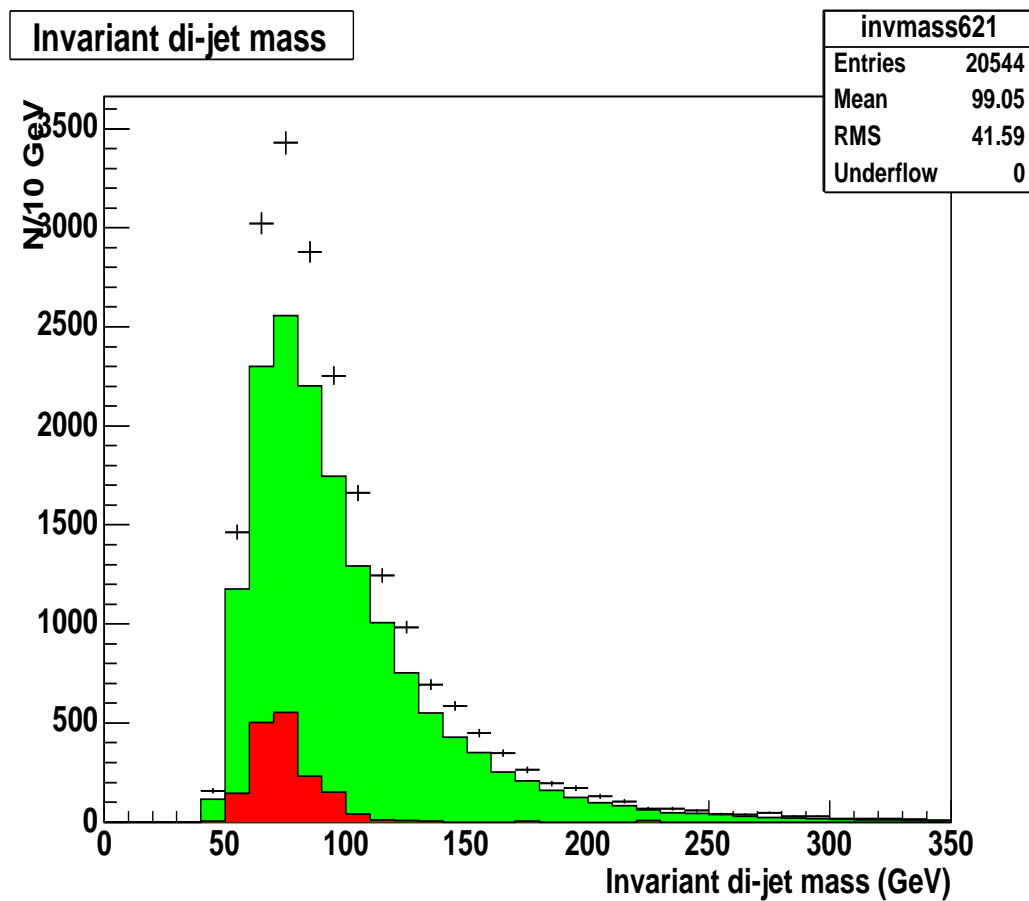
Figure 5.8: Invariant dijet mass in the pre-v13 data before background subtraction. Green (light grey) shaded histogram: expected background, estimated using the invariant mass-based TRF described in equation 5.2. Black points: total dijet mass distribution observed in pre-v13 data. Red (dark grey) shaded histogram: expected Z \rightarrow b\bar{b} signal from MC, weighted by cross-section and luminosity.
