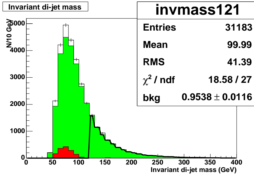
Figure B.6: Invariant dijet mass in the pre-v13 data before background subtraction. Green (light grey) shaded histogram: expected background, estimated using a jet-based TRF from in-zone events and fit to the observed data above 120 GeV/ c^2 . Black points: total dijet mass distribution observed in data. Red (dark grey) histogram: expected Z \rightarrow b\bar{b} signal from MC. The fit (bold black line) results in a correction to the background scale of 0.9538 \pm 0.0116 .
