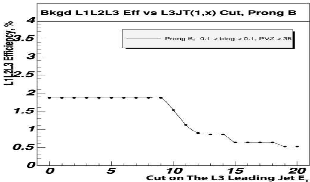
Figure 4.7: Background efficiency as a function of the cut on the leading jet E_T at Level 3. Trigger combination applied while the cut on the L3 jet E_T was varied: one L2 jet above 6 GeV, an L3 b -tag probability < 0.1 and an L3 primary vertex constraint of |z| < 35 cm.
