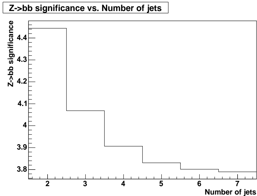
Figure 5.2: Effective signal significance, before cut 7 (the \Delta\varphi requirement), as a function of the cut on the number of good jets in the event ( n_{jet} ) in the pre-v13 data. The systematic error on the number of background events was set to 1% for the purposes of illustration. Maximum significance is obtained in events with two and only two jets.
