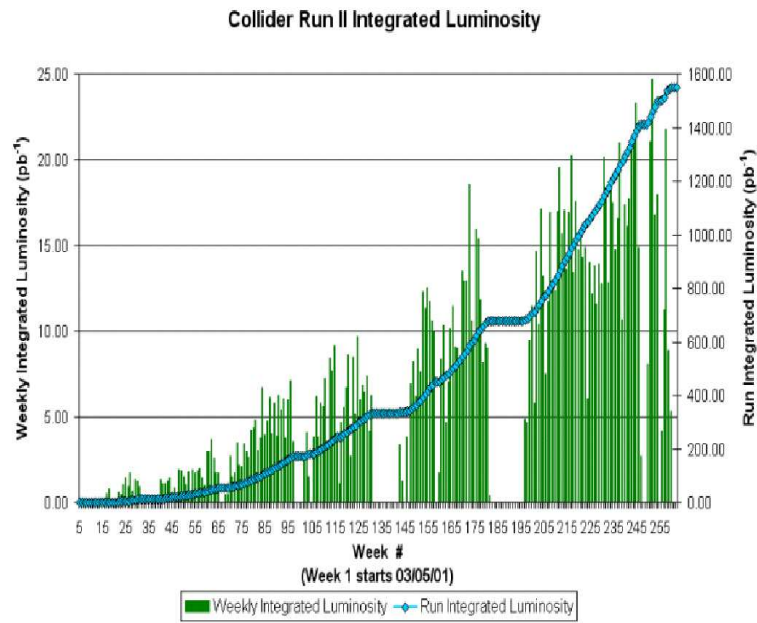
Figure 2.4: Integrated luminosity delivered by the Tevatron during Run II [27].
