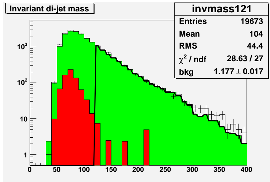
Figure B.2: Invariant dijet mass in the pre-v13 data before background subtraction. Green (light grey) shaded histogram: expected background, estimated using a jet-based TRF from out-of-zone events and fit to the observed data above 120 \text{ GeV}/c^2 . Black points: total dijet mass distribution observed in data. Red (dark grey) histogram: expected Z \rightarrow b\bar{b} signal from MC. The fit (bold black line) results in a correction to the background scale of 1.177 \pm 0.017 .
