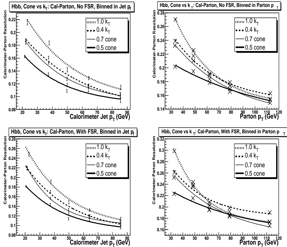
Figure 3.3: The effect of the jet algorithm on the b -jet resolution in ZH \rightarrow e^+e^-b\bar{b} . Comparisons were made at the calorimeter-parton level using uncorrected jets. Upper plots exclude hard FSR, lower ones include hard FSR. Binned in calorimeter jet p_T matched to partons (left) and in parton p_T before hard FSR (right).
