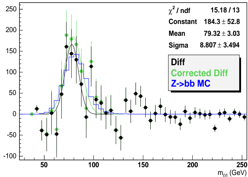
Figure 5.15: The final Z \rightarrow b\bar{b} peak derived from data, after explicit 0 \rightarrow 1 and signal corrections. Green (light grey) points: final distribution after all corrections. Blue (grey) line: the Z \rightarrow b\bar{b} MC peak. Black points: excess in data without the signal correction.
