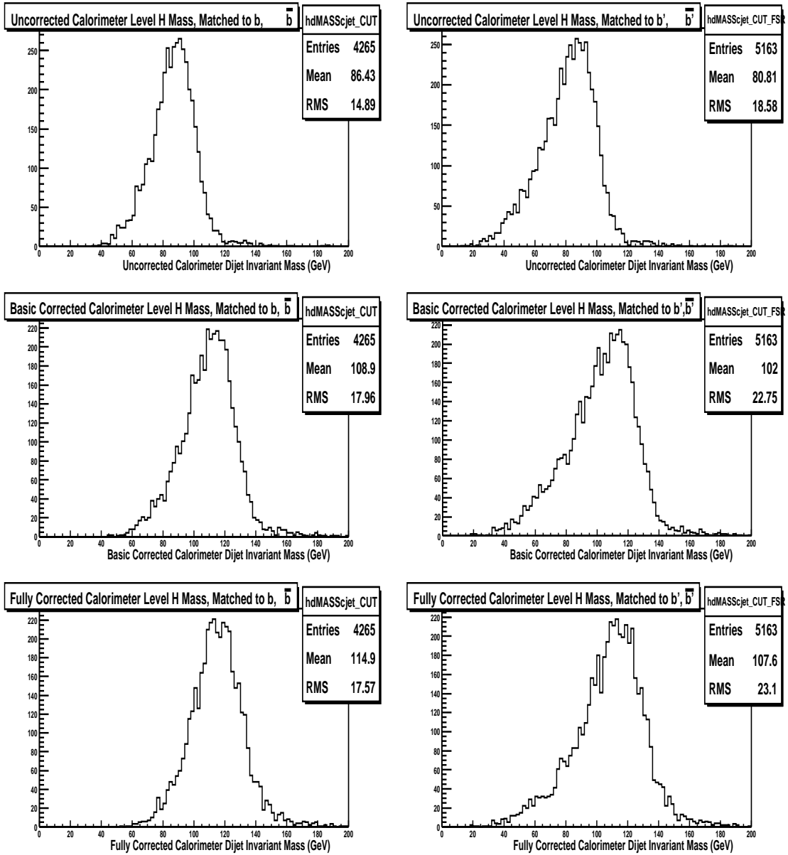
Figure 3.9: Reconstructed Higgs mass at calorimeter-jet level with no jet correction (top), basic correction (middle) and full, i.e. basic + muon, correction (bottom). Without hard FSR (left); with hard FSR (right). All jets are 0.5 cone.
