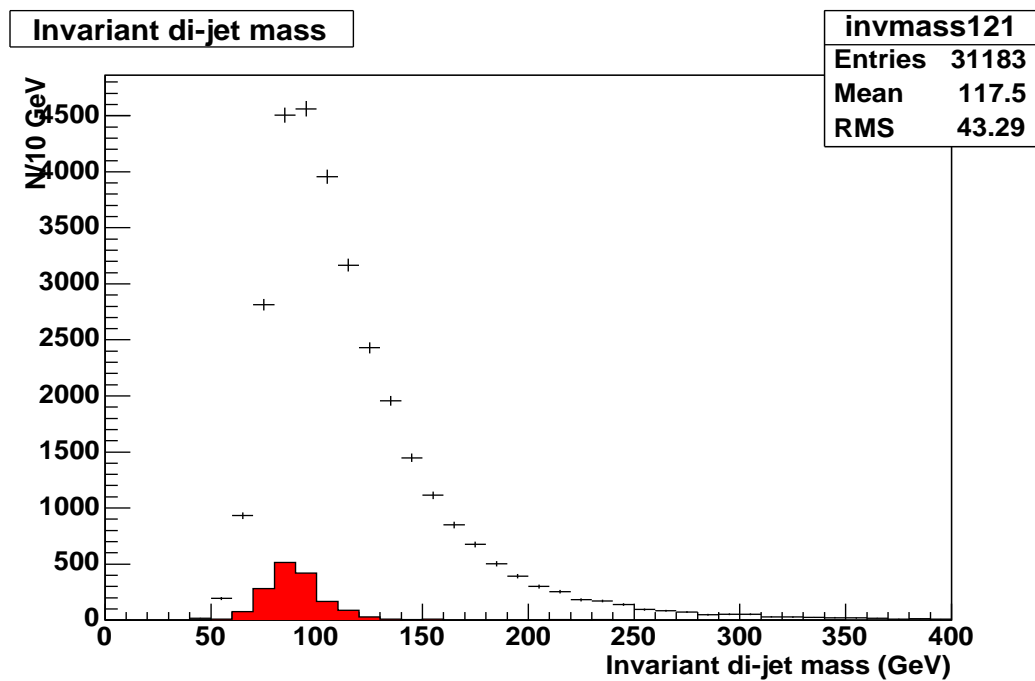
Figure 5.4: Comparison of the invariant di- b -jet mass in data and MC after event selection. Black points: pre-v13 data; red (grey) shading: expected Z \rightarrow b\bar{b} signal from MC. The region above 120 \text{GeV}/c^2 is almost signal-free.
