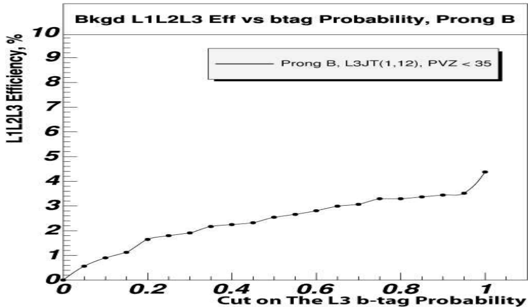
Figure 4.6: Background efficiency as a function of the cut on the L3 b -tag probability. The likelihood that the event is b -tagged increases as the probability approaches 0. Trigger combination applied while the cut on the b -tag probability was varied: one L2 jet above 6 GeV, one L3 jet above 12 GeV and an L3 primary vertex constraint of |z| < 35 cm.
