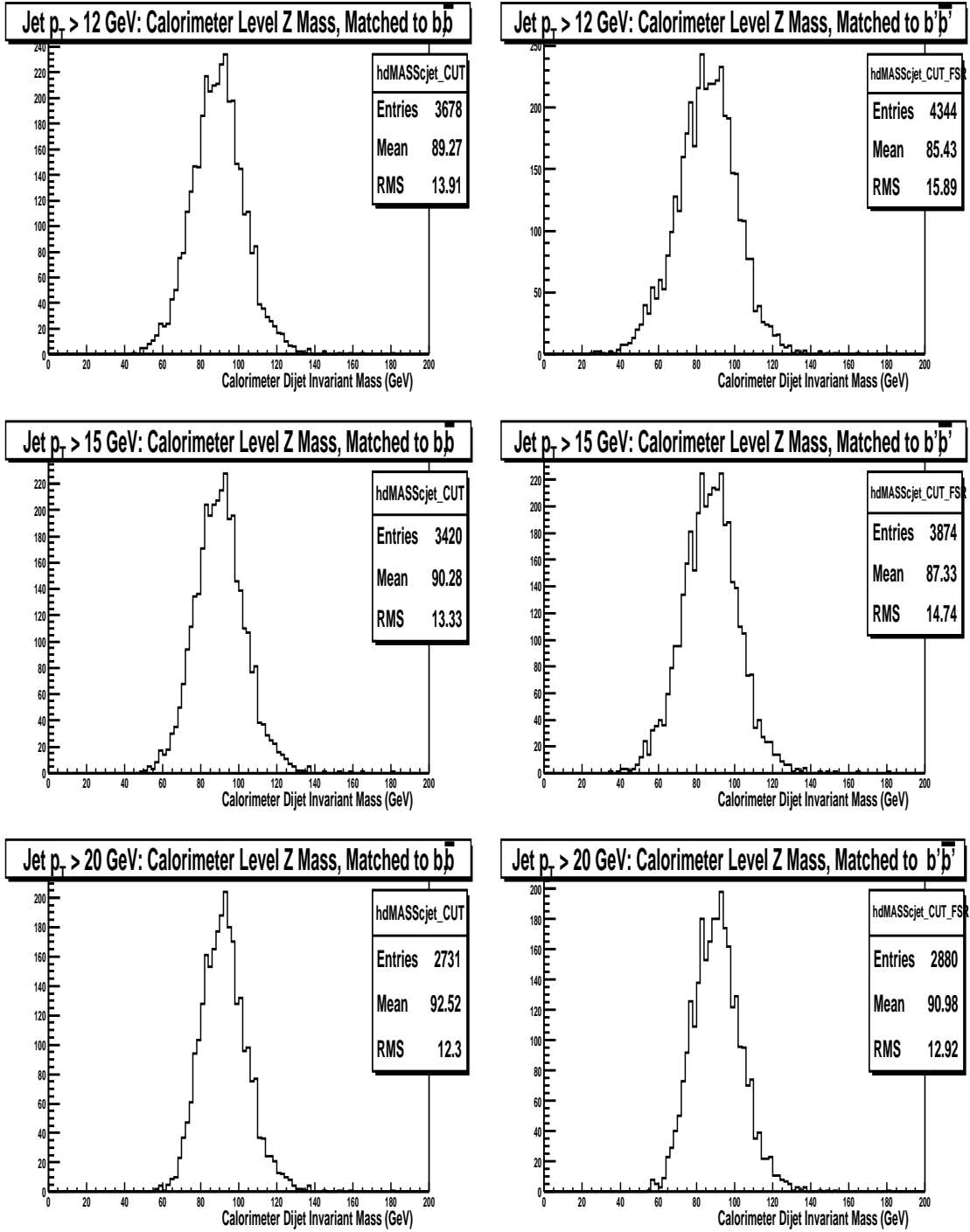
Figure 3.11: The effect of jet p_T cut on the Z dijet mass at calorimeter level. p_T cuts of 12 (top), 15 (middle), and 20 GeV/c (bottom) are shown, without hard FSR (left) and with hard FSR (right). Jets were 0.5 cone and full jet energy scale corrections were applied.
