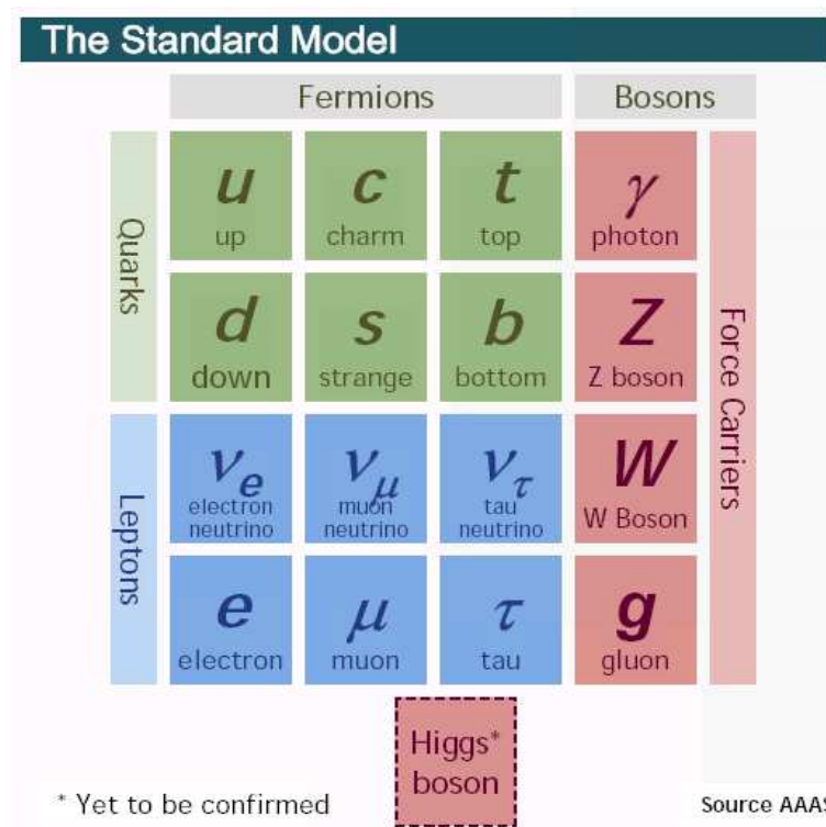
Figure 1.1: The Standard Model, which is a highly successful description of the subatomic world.
