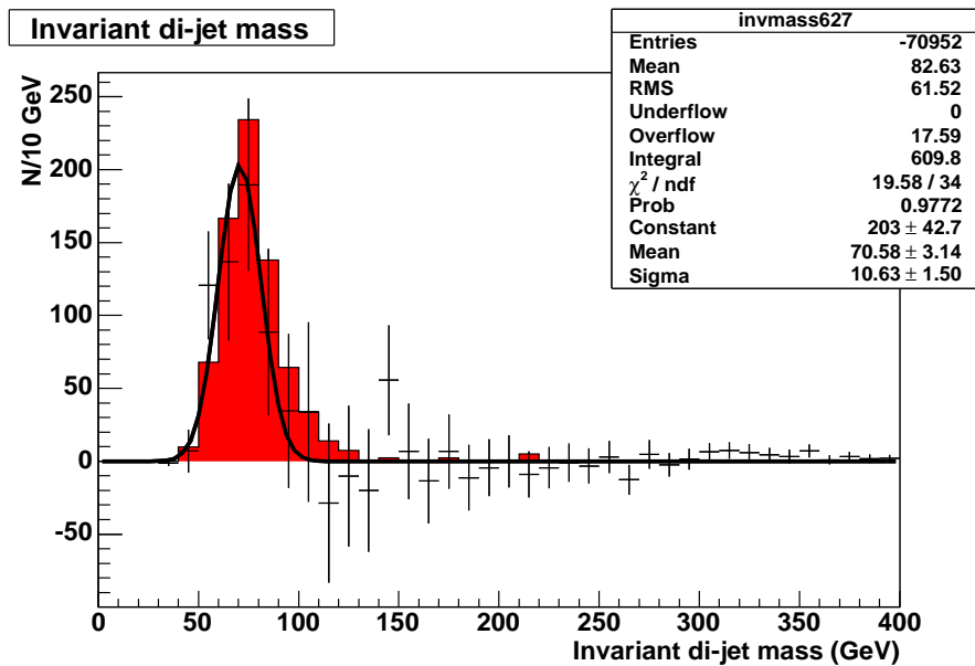
Figure B.4: Invariant dijet mass spectrum in the pre-v13 data after background subtraction (using the out-of-zone ( \Delta\varphi \leq 3.0 ) TRF). Black points: excess observed in data, fitted with a Gaussian. Error bars show statistical errors only. Red (dark grey) histogram: expected Z \rightarrow b\bar{b} signal from MC. The excess peak has a mean mass of 70.6 \text{ GeV}/c^2 and a width of 10.6 \text{ GeV}/c^2 .
