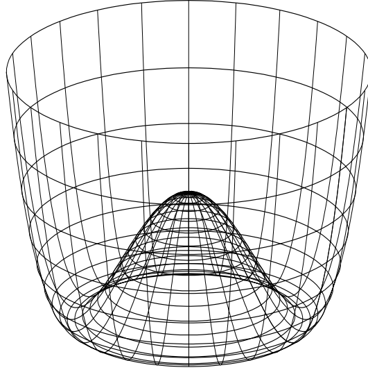
Figure 1.2: Graphical representation of the Higgs potential V(\phi) for the case in which \mu^2 is negative.
