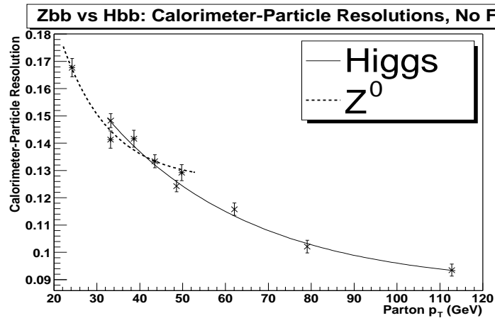
Figure 3.7: Comparison of Z and Higgs b -jet resolutions at calorimeter-particle level, excluding hard FSR. 0.5 cone corrected jets were used. Gaussian widths are plotted; error bars are statistical.
