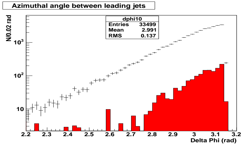
Figure 5.1: Comparison of the angular dijet distribution (delta phi or \Delta\varphi ) between pre-v13 data and Z \rightarrow b\bar{b} MC, after passing offline cuts 1–6. Red (dark grey) histogram: MC signal; black points: data. The signal is slightly more back-to-back than the background.
