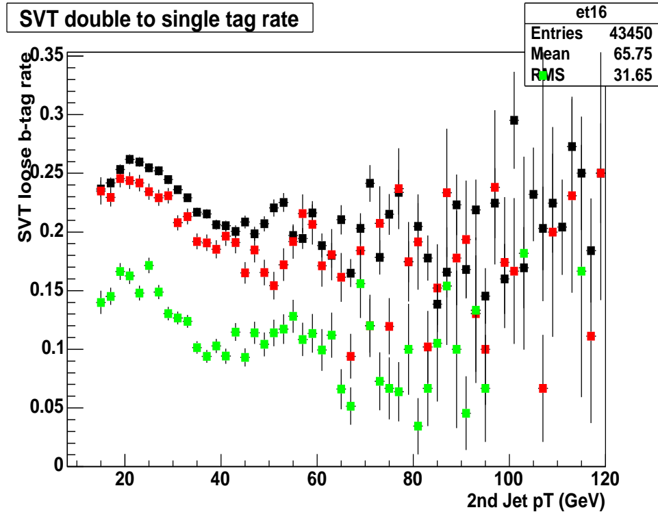
Figure B.5: Tag ratio as a function of second leading jet p_T for jets in the regions |\eta| < 1.1 (black), 1.1 < |\eta| < 1.5 (red (medium grey)) and 1.5 < |\eta| < 2.5 (green (light grey)), evaluated for in-zone ( \Delta\varphi > 3.0 ) events in pre-v13 data.
