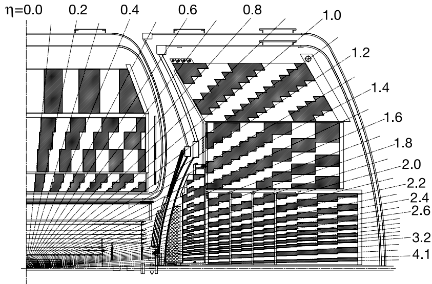
Figure 2.11: Side view of a quadrant of the calorimeter, in the y - z plane. The central barrel and end cap of the calorimeter can be seen in separate cryostats. The labels designate projected values of \eta .
