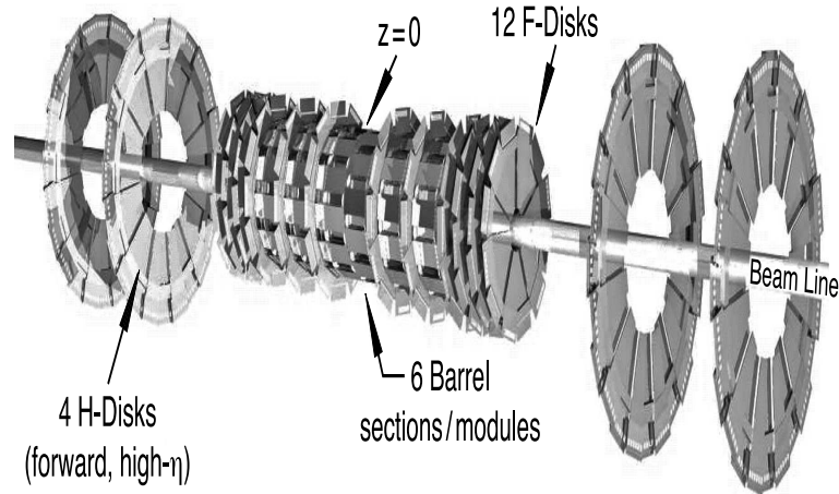
Figure 2.9: Three-dimensional view of the SMT. The six central barrels surround the proton-antiproton interaction region (a 1 metre region of z space). Beyond this, the twelve F-Disks and four H-Disks can be seen.
