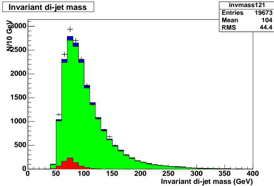
Figure B.3: Invariant dijet mass in the pre-v13 data before background subtraction. Green (light grey) shaded histogram: expected background, estimated using a jet-based TRF from out-of-zone events. The dark blue (black) band represents the \pm 1.5\% systematic error on the background from the normalisation fit. Black points: total dijet mass distribution observed in data. Red (dark grey) histogram: expected Z \rightarrow b\bar{b} signal from MC.
