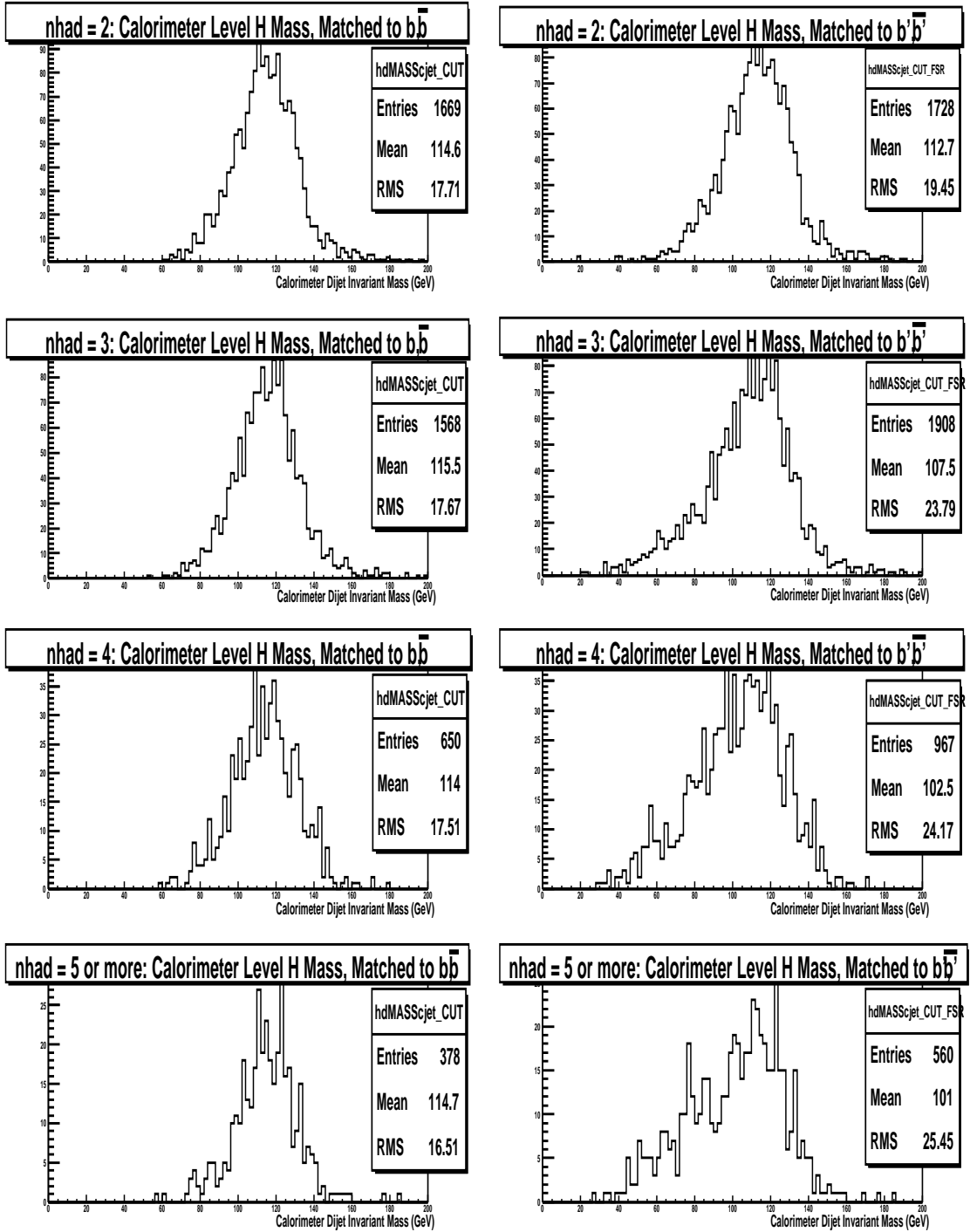
Figure 3.10: The effect of jet multiplicity on the Higgs mass resolution at calorimeter level. From top to bottom: n_{had} = 2 ; n_{had} = 3 ; n_{had} = 4 ; n_{had} \geq 5 . Without hard FSR (left); with hard FSR (right). All jets are 0.5 cone, no jet p_T cuts were imposed and full jet energy scale corrections were applied.
