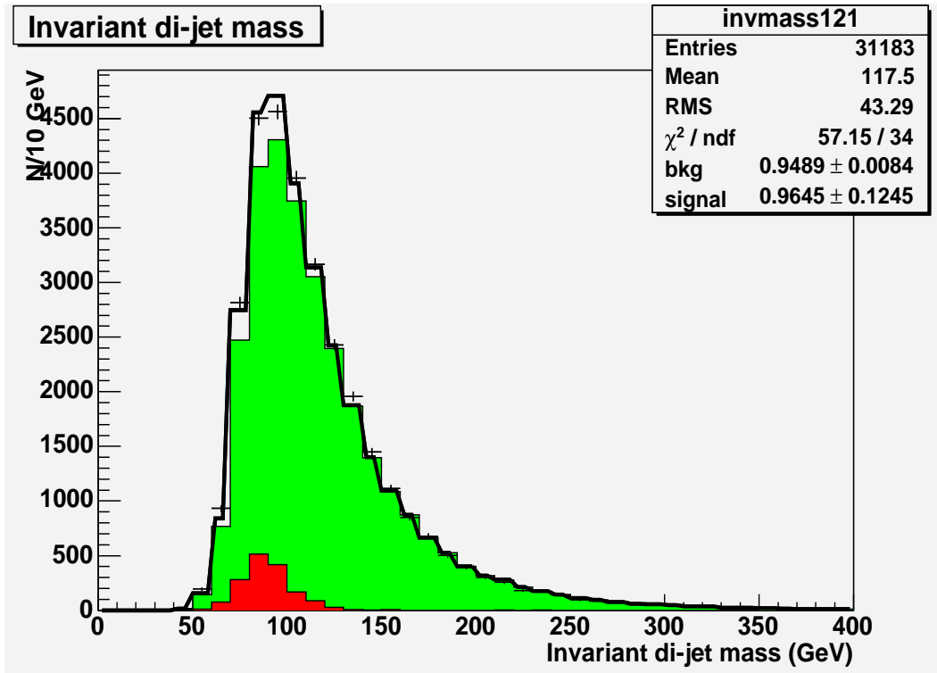
Figure 5.14: Closure test of the final invariant dijet mass spectrum observed in the pre-v13 data after background subtraction. Green (light grey) shaded histogram: expected background, estimated using a jet-based TRF from in-zone events. Black points: total dijet mass distribution observed in data. Red (dark grey) shaded histogram: expected signal from MC. The bold black line shows the fitted sum of the scaled background and MC templates.
