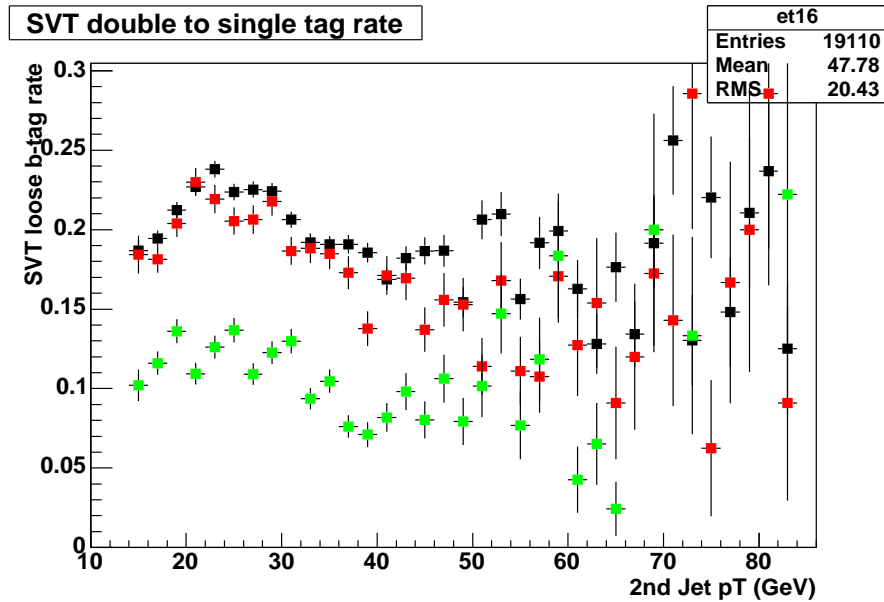
Figure B.1: Tag ratio as a function of second leading jet p_T for jets in the regions |\eta| < 1.1 (black), 1.1 < |\eta| < 1.5 (red (medium grey)) and 1.5 < |\eta| < 2.5 (green (light grey)), evaluated for out-of-zone ( \Delta\varphi \leq 3.0 ) events in pre-v13 data.
