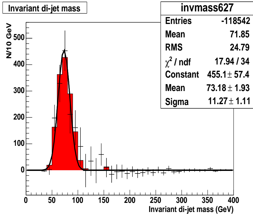
Figure B.8: Invariant dijet mass spectrum in the pre-v13 data after background subtraction (using the in-zone TRF). Black points: excess observed in data, fitted with a Gaussian. Error bars show statistical errors only. Red (dark grey) histogram: expected Z \rightarrow b\bar{b} signal from MC. The excess peak has a mean mass of 73.2 \text{ GeV}/c^2 and a width of 11.3 \text{ GeV}/c^2 .
