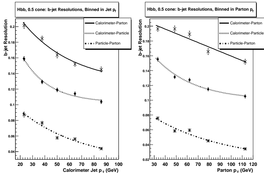
Figure 3.2: b -jet resolution as a function of p_T for ZH \rightarrow e^+e^-b\bar{b} , without hard FSR. The lines shown are there to guide the eye, however they are fits to the data obtained using a fit form given by equation 3.9. The fit is performed for all three lines on each graph even though equation 3.9 contains noise terms that don't apply to the particle-parton case. Resolution is binned in calorimeter jet p_T before hard FSR (left) and b parton p_T before hard FSR (right). All calorimeter jets are fully corrected.
