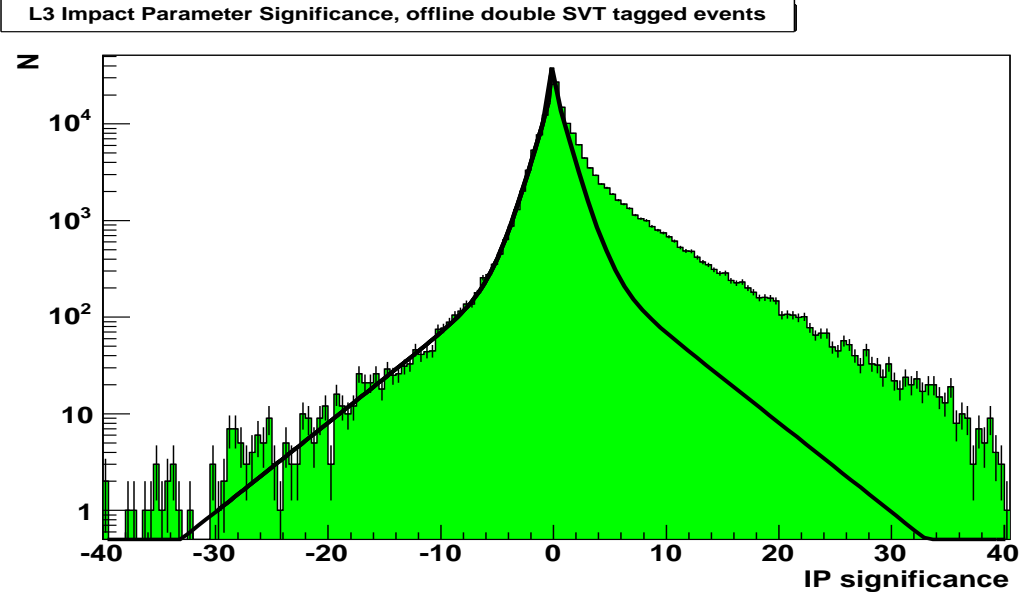
Figure 4.4: Signed impact parameter distribution from data events that contain two offline b -tags. The excess seen in the right-hand tail comes from b -tagged events. The bold black line shows a fit to the negative side of the distribution (IP significance < 0 ) folded over to the positive side.
