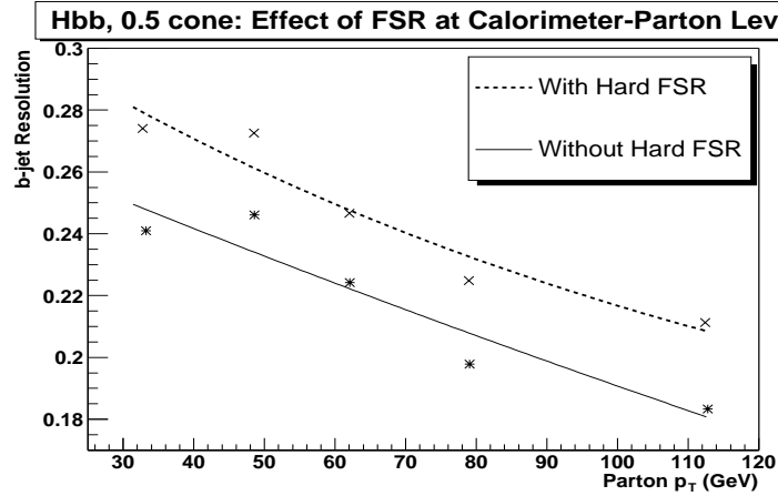
Figure 3.6: Effect of hard FSR on b -jet resolution in ZH \rightarrow e^+e^-b\bar{b} at the particle-parton level.
