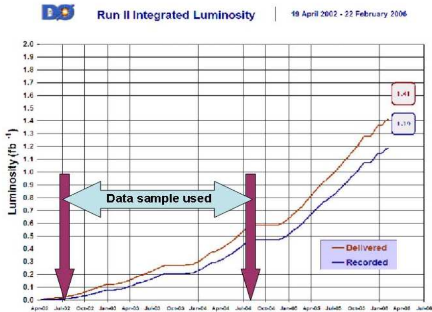
Figure 2.14: Integrated luminosity collected by the DØ experiment up to 22 February 2006, when the latest accelerator shutdown began [35].
