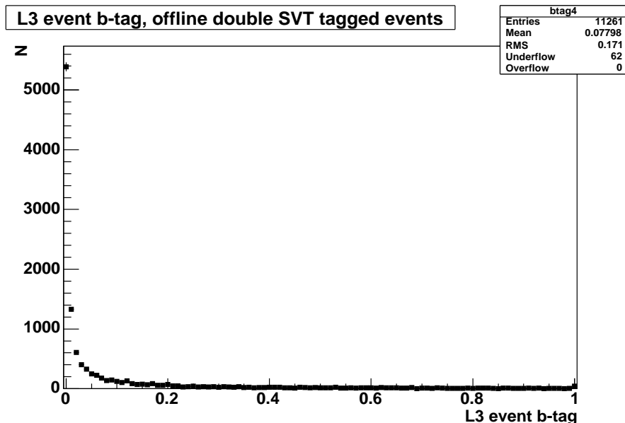
Figure 4.5: Level 3 event b -tag probability for data events that have two offline b -tags. The narrow peak near 0 indicates that the sample is rich in b -content.
