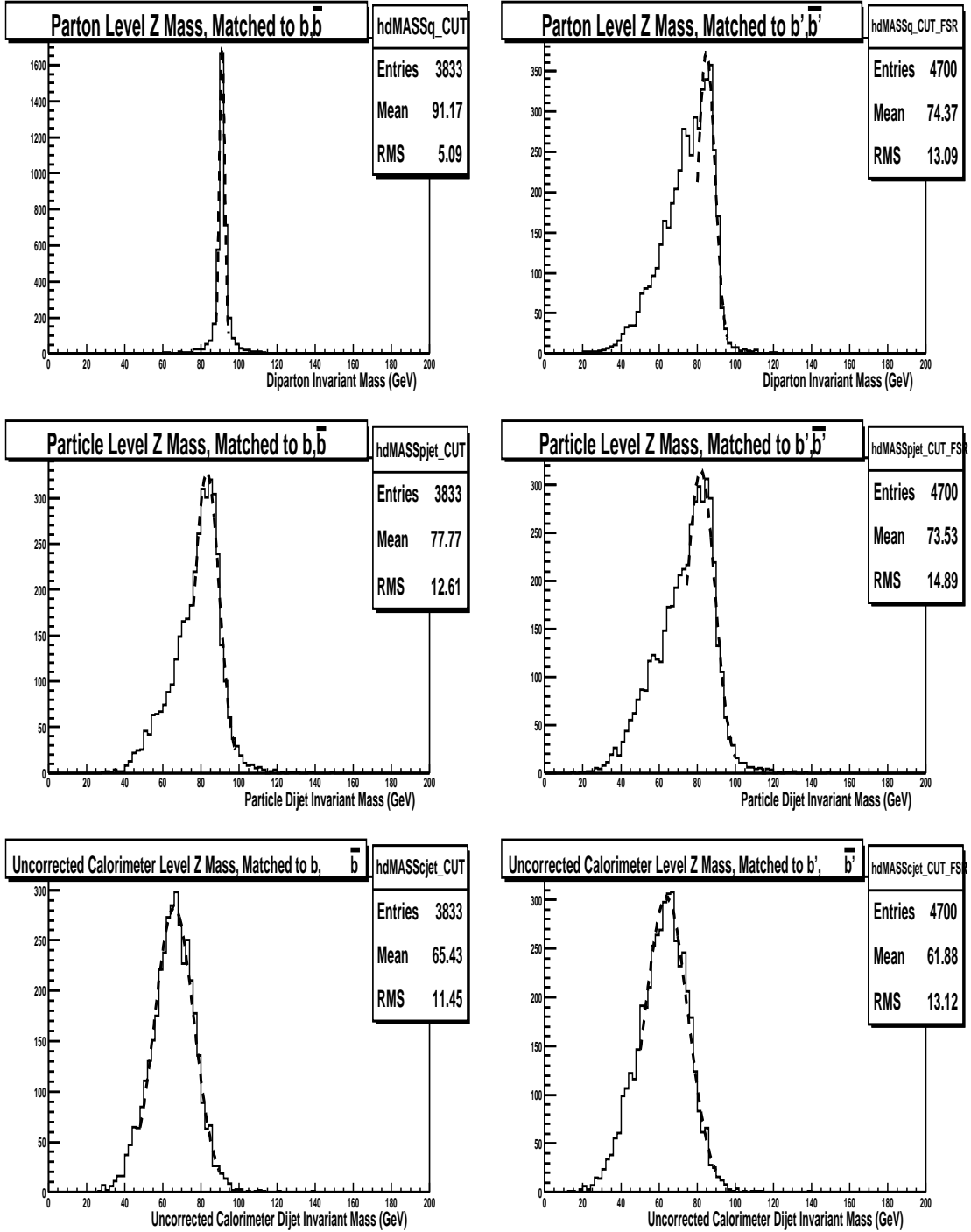
Figure A.1: Reconstructed Z mass at parton (top), particle-jet (middle) and uncorrected calorimeter-jet (bottom) levels. Without hard FSR (left); with hard FSR (right). All jets are 0.5 cone. Dashed profiles show central Gaussian fits to each distribution.
