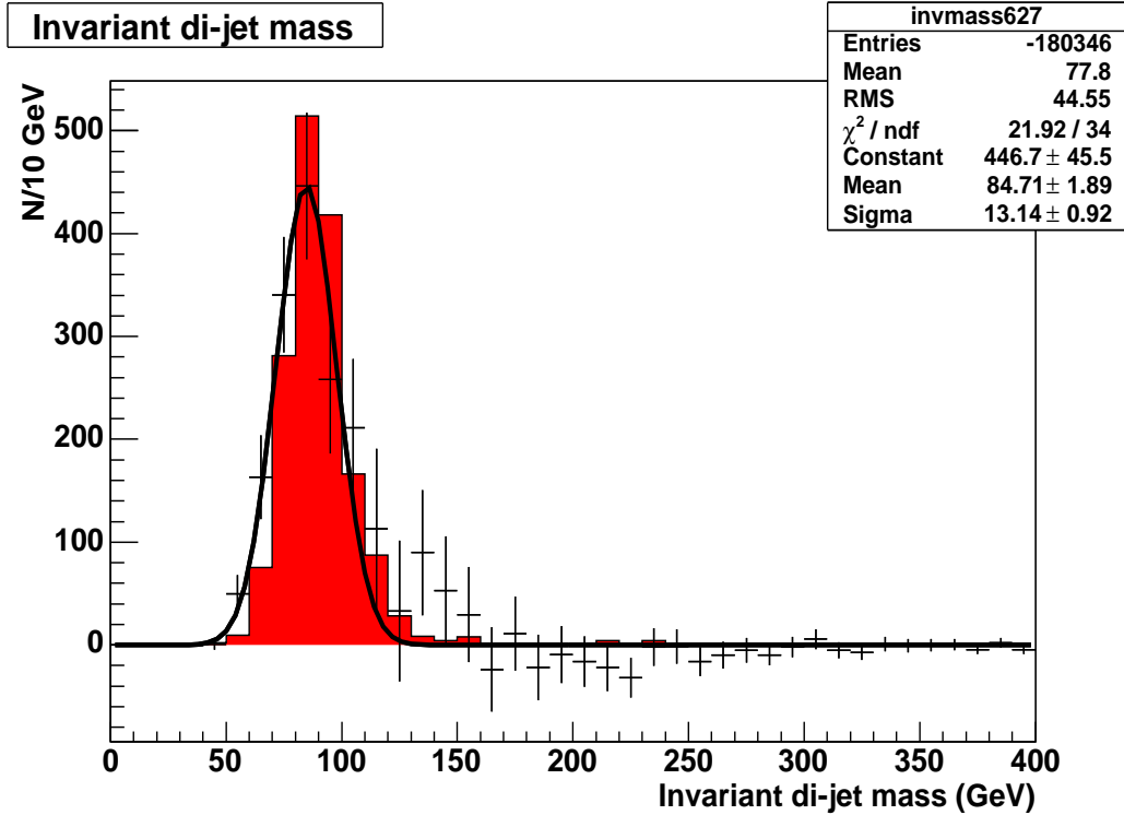
Figure 5.13: Invariant dijet mass spectrum in the pre-v13 data after background subtraction (using the in-zone, \Delta\varphi > 2.75 , jet-based TRF). Black points: excess observed in data, fitted with a Gaussian. Error bars show statistical errors only. Red (dark grey) histogram: expected Z \rightarrow b\bar{b} signal from MC. The excess peak has a mean mass of 84.7 \text{ GeV}/c^2 and a width of 13.1 \text{ GeV}/c^2 .
