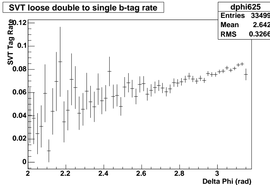
Figure 5.9: The variation of tag ratio with \Delta\varphi between the two leading b -jets in each event, for pre-v13 data, using jets from all \eta regions. A linear dependence of the tag ratio upon \Delta\varphi is observed.
