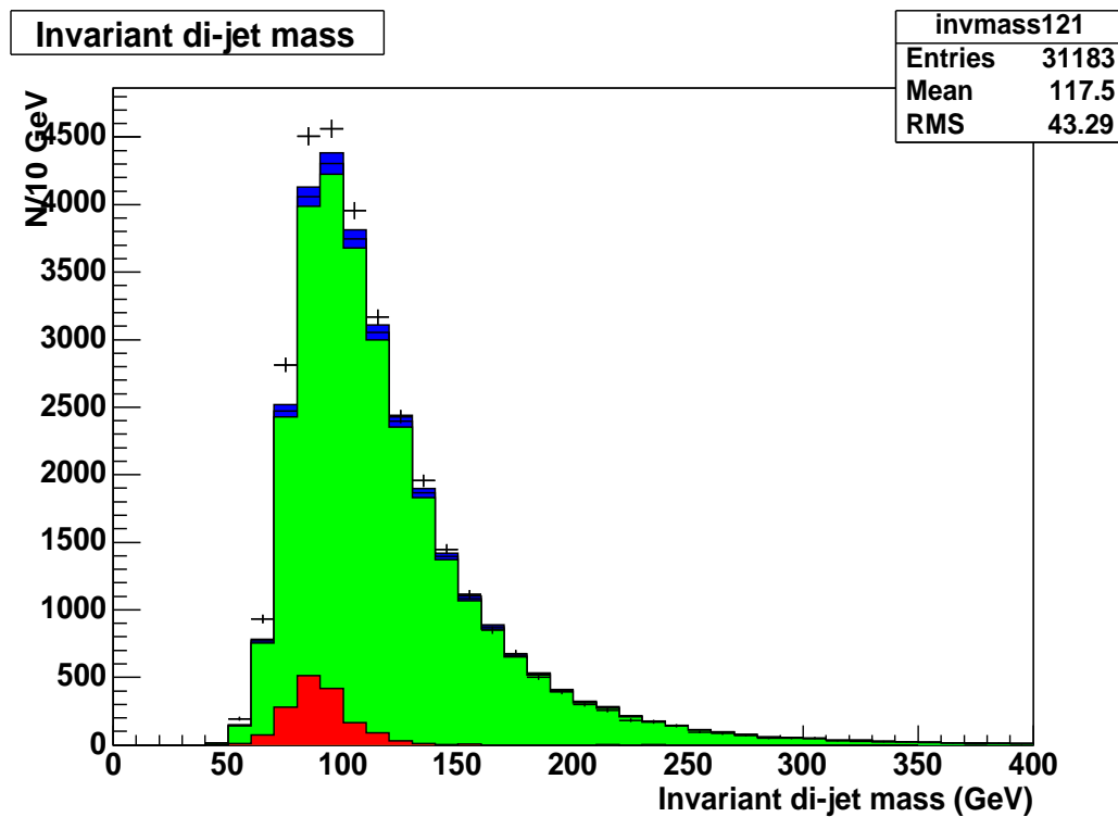
Figure 5.12: Invariant dijet mass in the pre-v13 data before background subtraction. Green (light grey) shaded histogram: expected background, estimated using a jet-based TRF from in-zone ( \Delta\varphi > 2.75 ) events. The dark blue (black) band represents an overall systematic error on the background of \pm 1.8\% , discussed in Section 5.6.6. Black points: total dijet mass distribution observed in data. Red (dark grey) shaded histogram: expected Z \rightarrow b\bar{b} signal from MC.
