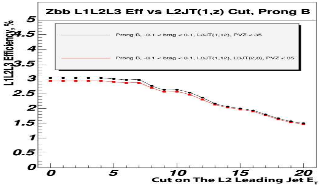
Figure 4.13: Signal efficiency as a function of jet E_T cut applied at Level 2. Black circles (upper line): b -tag constraint plus primary vertex cut applied at L3, with a cut on the leading L3 jet of 12 GeV. Red squares (lower line): same as upper line with an additional cut of 8 GeV on the second leading L3 jet.
