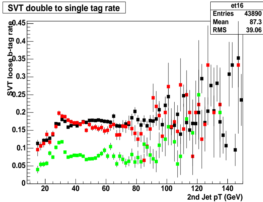
Figure 5.10: Tag ratio as a function of second leading jet p_T for jets in the regions |\eta| < 1.1 (black), 1.1 < |\eta| < 1.5 (red (medium grey)) and 1.5 < |\eta| < 2.5 (green (light grey)), evaluated for in-zone events in pre-v13 data.
