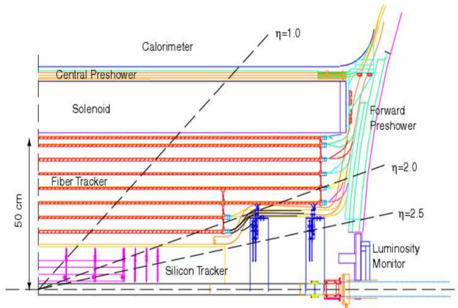
Figure 2.8: Side view of a quadrant of the tracking system in relation to the preshower detectors and calorimeter.
