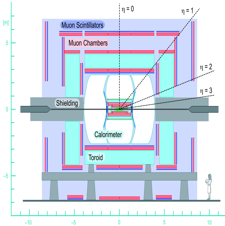
Figure 2.6: Side view of the DØ Run II detector. From the interaction point outward one can see the Silicon Microstrip Tracker (SMT) and Central Fibre Tracker (CFT) tracking components with their solenoid magnet, surrounded by the calorimeter in its three cryostats and the muon system with its toroidal magnet.
