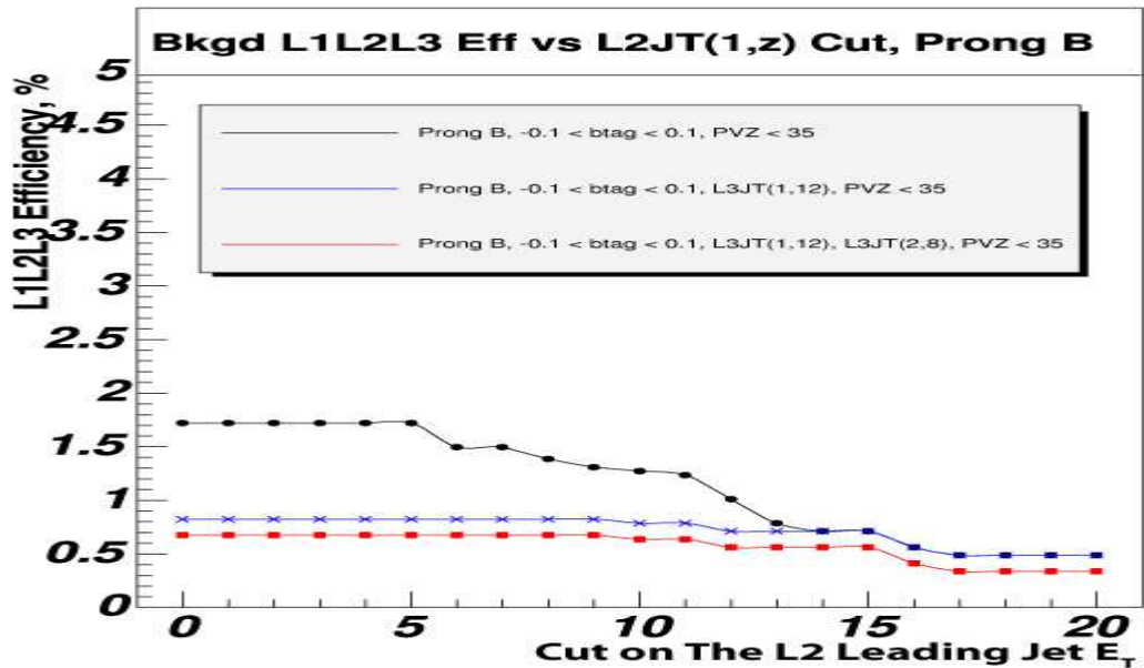
Figure 4.9: Background efficiency as a function of the cut on the jet E_T at Level 2. Black circles (upper line): b -tag constraint plus primary vertex cut applied at L3. Blue crosses (middle line): same as upper line, with an extra E_T cut on the leading L3 jet of 12 GeV. Red squares (bottom line): same as middle line with a cut of 8 GeV on the p_T of the second leading jet at L3.
