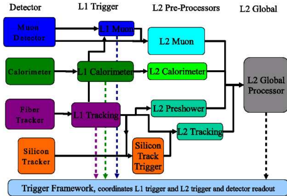
Figure 2.13: Block diagram of the DØ L1 and L2 trigger systems. Horizontal arrows represent the net flow of physics information through the detector. Vertical arrows symbolise the flow of data to the trigger framework, which then makes global L1 and L2 trigger decisions ready to pass to L3.
