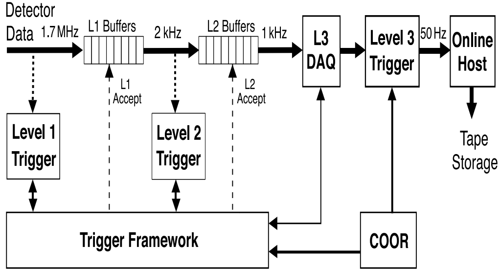
Figure 2.12: Overview of the DØ trigger and data acquisition (DAQ) systems [21]. Overall coordination and control of DØ triggering is controlled by a package known as ‘COOR’ that runs on the online host machine.
