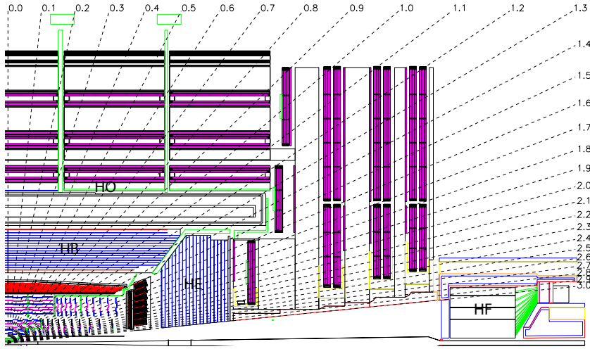
Figure 2.10.: A schematic of one quadrant of the CMS HCAL showing the barrel (HB), outer (HO), endcap (HE) and forward (HF) regions. Taken from [56].
