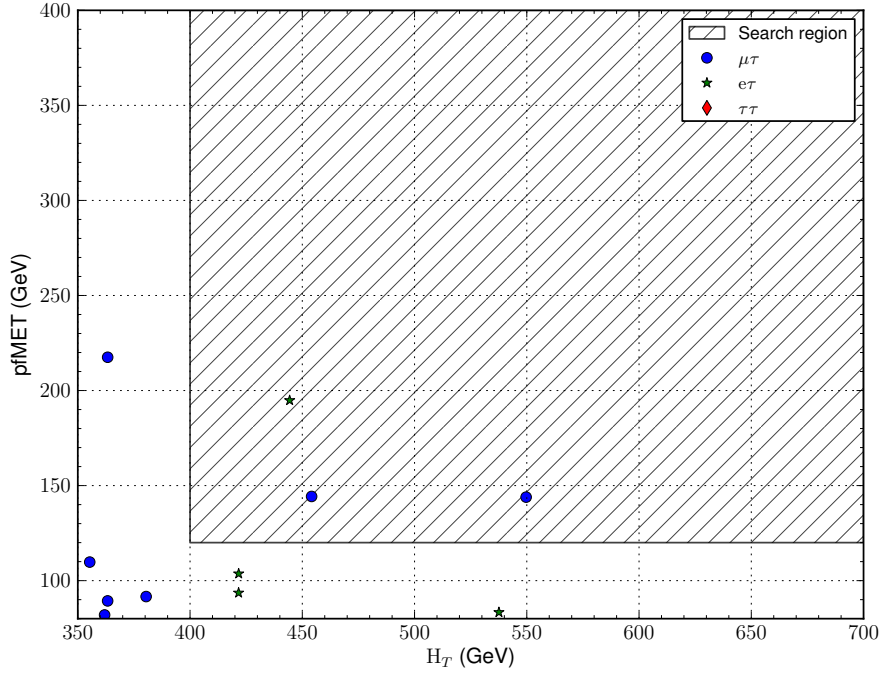
Figure 6.1.: Scatter plot of the \tau SSDL events passing the full signal selection in data in the H_T -pfMET plane. The region outside the search region is below the trigger efficiency for the data taken in the 2 \times 10^{33} \text{ cm}^{-2} \text{ s}^{-1} regime.
