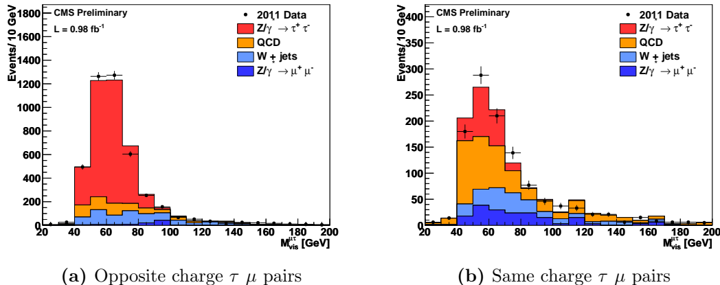
Figure 5.5.: Invariant mass distributions of \mu\tau for opposite (5.5a) and same-sign (5.5b) charges, computed using the visible \tau momentum. Data points and MC signal and background expectation is shown. The shapes of the signal and background are taken from MC and fitted to the data to determine their relative scales.
