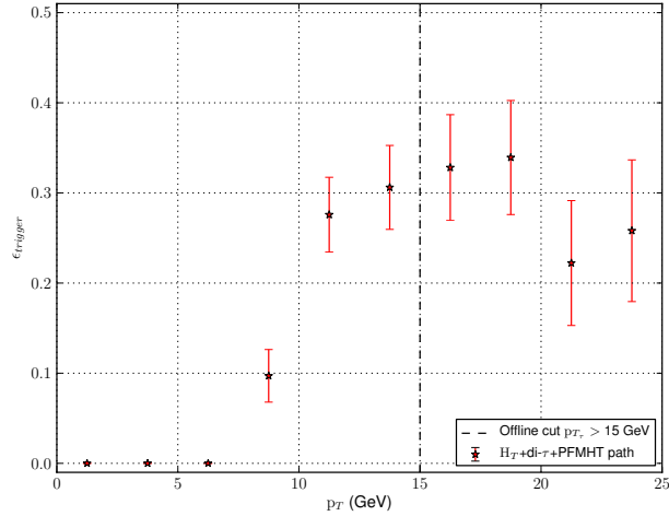
(b) SSDL \tau trigger p_T turn-on.
