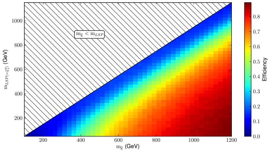
(b) Efficiency after E_T^{miss} request.
