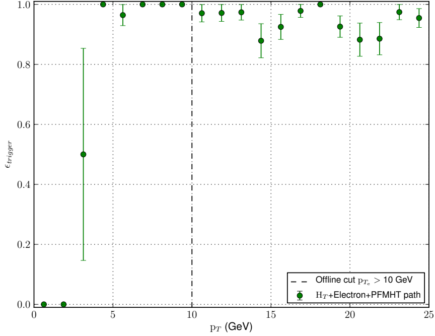
(a) Electron trigger offline p_T turn-on.
