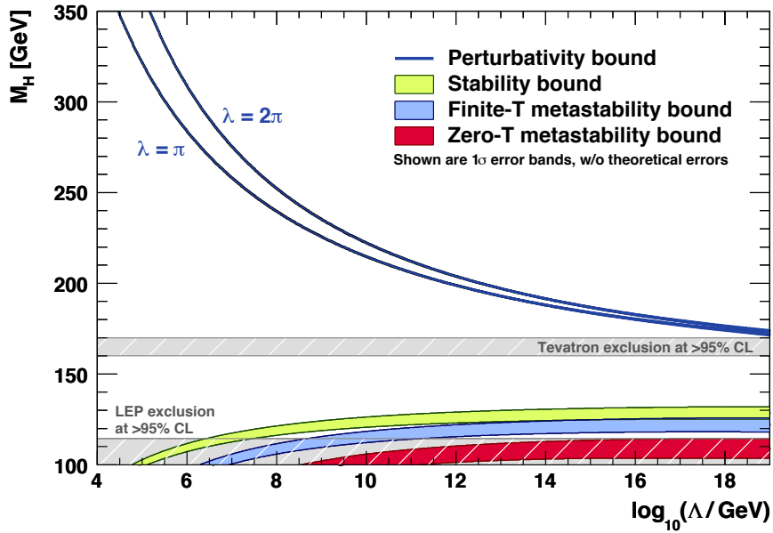
Figure 1.1.: Bounds on the Higgs mass from perturbative and stability arguments, as a function of energy scale \Lambda . Widths of the bands show uncertainties. The exclusions on the Higgs mass from the Tevatron and LEP experiments are shown. A description of the Finite-T and Zero-T metastability bounds may be found in [28]. Taken from [28].
