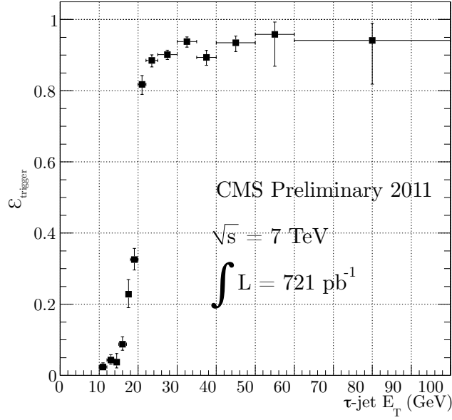
(a) Example \tau trigger E_T turn-on. Taken from [83].
