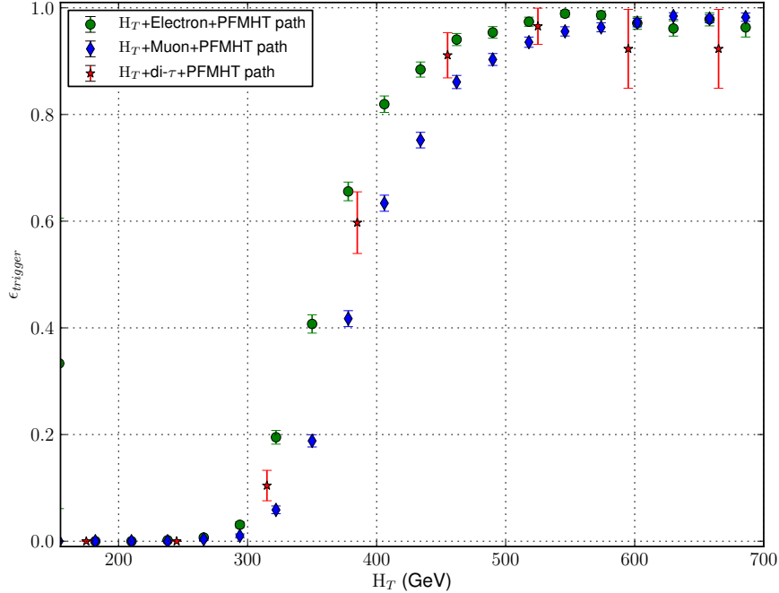
Figure 4.4.: Offline H_T turn-on in the 1 \times 10^{33} \text{ cm}^{-2} \text{ s}^{-1} regime for all three trigger paths with H_T > 250 GeV in the denominator and H_T > 350 GeV in the numerator. This set of trigger paths (with H_T > 350 GeV) was not used in the presented analysis.
