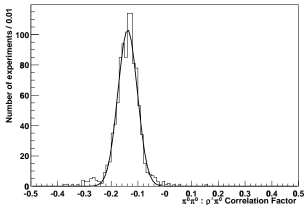
Figure 5.16: An example of the fit correlation for the B^0 \rightarrow \pi^0\pi^0 and B^\pm \rightarrow \rho^\pm\pi^0 components taken from 1000 toy Monte Carlo experiments. The distribution is fitted with a Gaussian and the correlation is extracted from the Minuit correlation matrix once the fit has been performed. The mean of the fitted Gaussian is -0.14 , and the RMS of the distribution is 0.04 .
