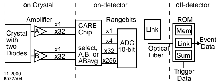
Figure 2.20: EMC read out design
