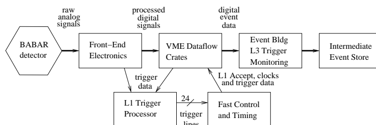
Figure 2.27: Schematic diagram of the BABAR DAQ system.
