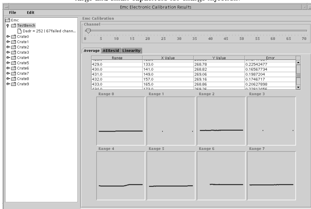
Figure 3.3: Output of the modified odd-even electronics calibration GUI for a non-pulsed channel. The 8 ranges correspond to the \times 1 (0&1), \times 4 (2&3), \times 32 (4&5), and \times 256 (6&7) electronics ranges using the large and small capacitors for charge injection.
