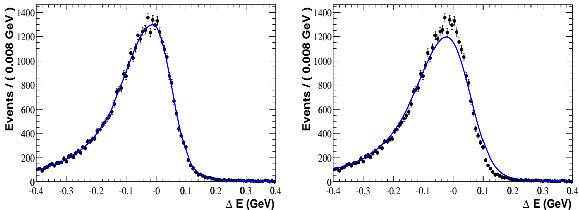
Figure 5.17: The B^0 \rightarrow \pi^0\pi^0 \Delta E distribution with the generated Keys PDF overlayed for a Keys PDF generated using a small ( 0.3\times nominal) Gaussian bandwidth (left) and a larger ( 1.6\times nominal) Gaussian bandwidth (right).
