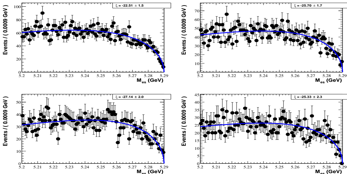
Figure 5.12: On-resonance m_{ES} distributions showing the variation in the fitted \xi Argus parameter. The top left plot corresponds to the \Delta E range ( -0.4 < \Delta E < -0.2 GeV), top right to ( -0.2 < \Delta E < 0.0 GeV), bottom left to ( 0.0 < \Delta E < 0.2 GeV) and bottom right to ( 0.2 < \Delta E < 0.4 GeV). A cut on \mathcal{F} was applied to remove over 90% of the B^0 \rightarrow \pi^0 \pi^0 and B^\pm \rightarrow \rho^\pm \pi^0 events in the sample.
