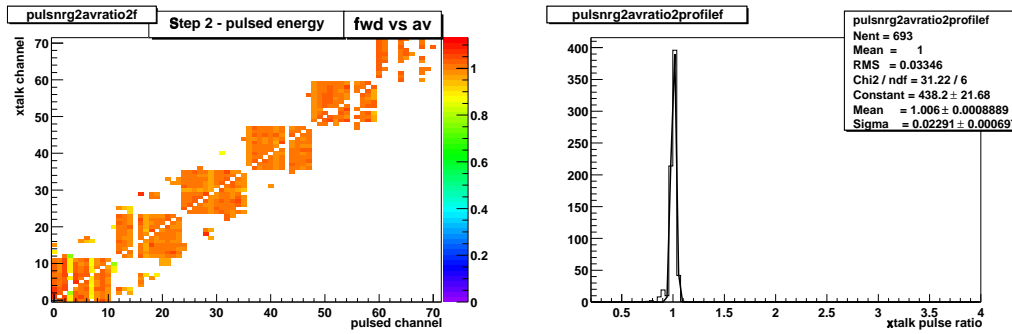
Figure 3.18: The ratio of the forward barrel Pulse 2 measurements to the averaged barrel Pulse 2 measurements. The plot shows which minirate readout channels see induced signals from the different pulsed channels within the minirate. A minimum \Delta_2 energy cut is applied to get rid of fake signals due to noise and individual failed calibrations.
