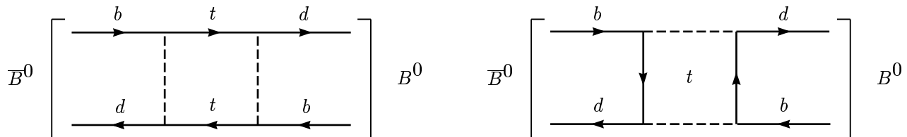
Figure 1.1: Box diagrams for B^0 - \bar{B}^0 mixing in the Standard Model.
