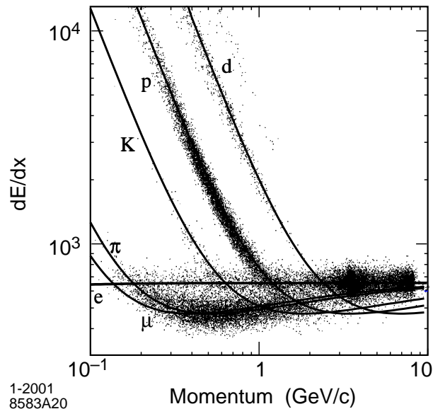
Figure 2.12: DCH dE/dx distribution for data as a function of track momentum. The expected Bethe-Bloch distributions for e^\pm, \mu^\pm, \pi^\pm , and K^\pm, p and d are overlaid. The dE/dx units are given by \text{keV}/m .
