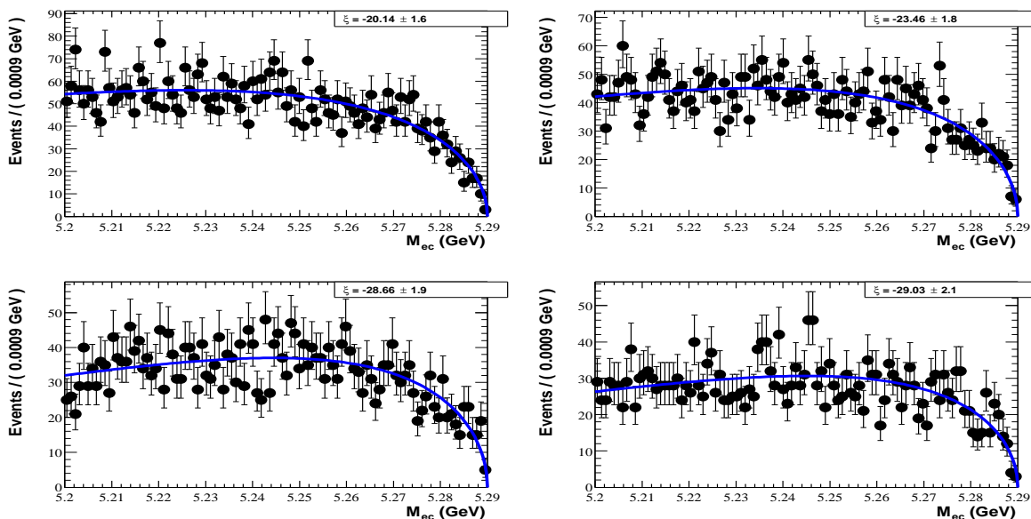
Figure 5.13: On-resonance m_{EC} distributions showing the variation in the fitted \xi Argus parameter. The top left plot corresponds to the \Delta E range ( -0.4 < \Delta E < -0.2 GeV), top right to ( -0.2 < \Delta E < 0.0 GeV), bottom left to ( 0.0 < \Delta E < 0.2 GeV) and bottom right to ( 0.2 < \Delta E < 0.4 GeV). A cut on \mathcal{F} was applied to remove over 90% of the B^0 \rightarrow \pi^0 \pi^0 and B^\pm \rightarrow \rho^\pm \pi^0 events in the sample.
