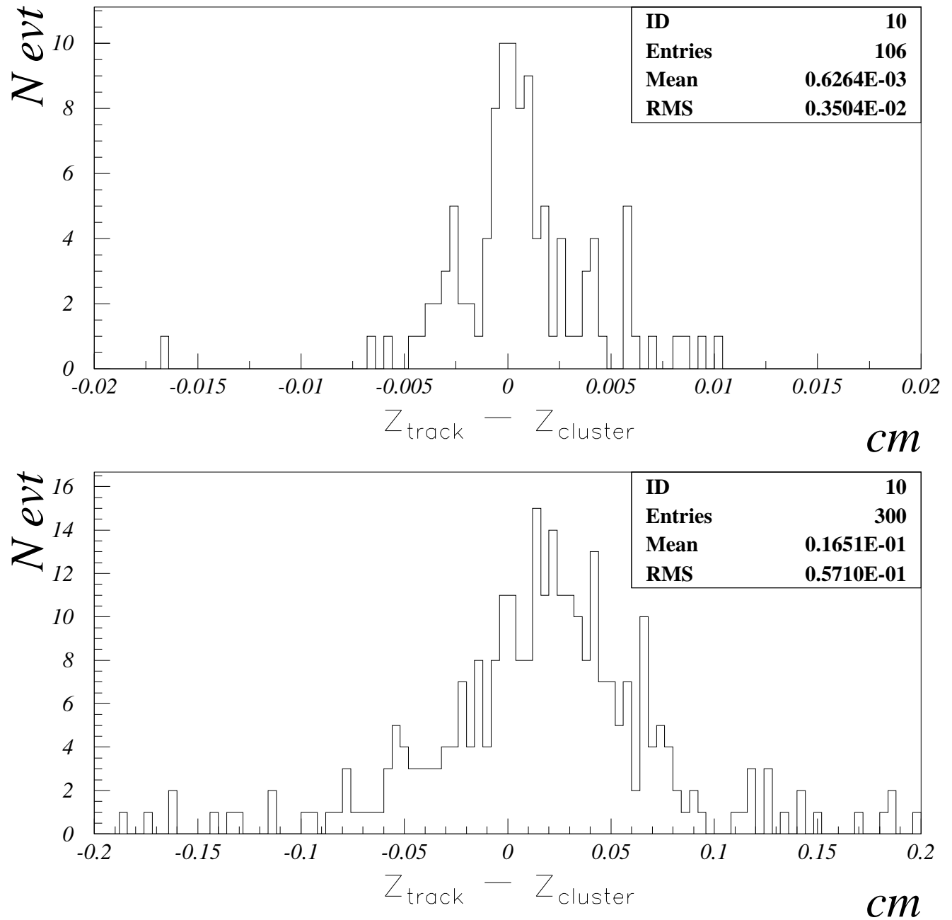
Figure 4.21: Resolution in z (top: 90^\circ , bottom: 2^\circ ) from offline reconstruction [57].
