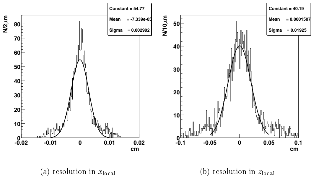
Figure 4.10: Spatial resolution for H-Disks. Plotted is the difference between the Monte Carlo and the reconstructed cluster position for each reconstructed cluster.
