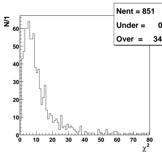
Figure 5.15: \chi^2 distribution for selected B_s^0 candidates within 0.06 \text{ GeV} ( \approx 2\sigma ) of the nominal B_s^0 mass. The four track fit has five degrees of freedom. Candidates had to pass all cuts listed in table 5.2, except for the B_s^0 \chi^2 cut. If more than one candidate per event passed all cuts, only the candidate with the smallest \chi^2 was kept.
