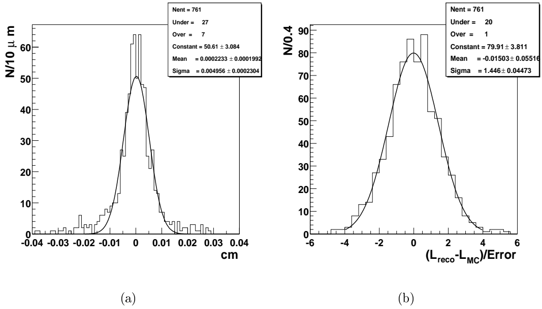
Figure 5.22: (a) Proper decay length resolution (reconstructed proper decay length - MC proper decay length) for B_s^0 \rightarrow J/\psi \phi . If the event was a background event the MC proper decay length was set to 1000.0 which causes the excess of events in the underflow bin. (b) Difference between the MC proper decay length and the reconstructed proper decay length divided by the error on the proper decay length according to eq. 5.5. In both histograms a Gaussian was fitted.
