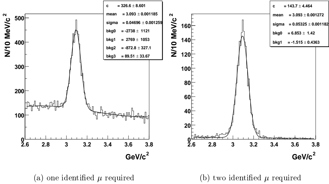
Figure 5.5: Invariant mass distribution for all J/\psi candidates in the signal sample. The fitted function in (a) is a Gaussian and a third order polynomial, the function in (b) a Gaussian and a straight line. The peak in (a) contains approximately twice as many J/\psi candidates as the peak in (b).
