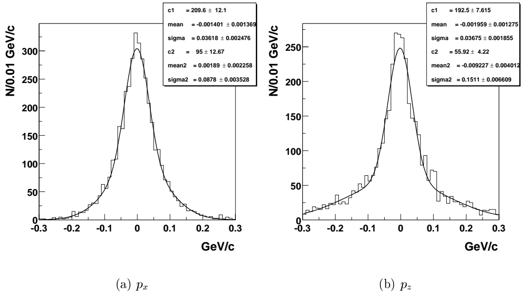
Figure 5.8: J/\psi momentum resolution in p_x and p_z . The fitted function is a double Gaussian.
