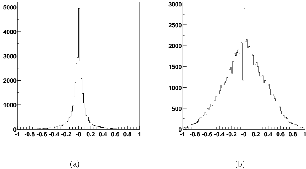
Figure 4.4: Example distributions of the energy ratio \frac{e_1 - e_2}{e_1 + e_2} for real hits (a) and ghosts (b). Note that ghost-killing will not reduce the number of fake clusters due to multiplexing in the 90^\circ stereo layers. The spike in (b) is due to rounding errors.
