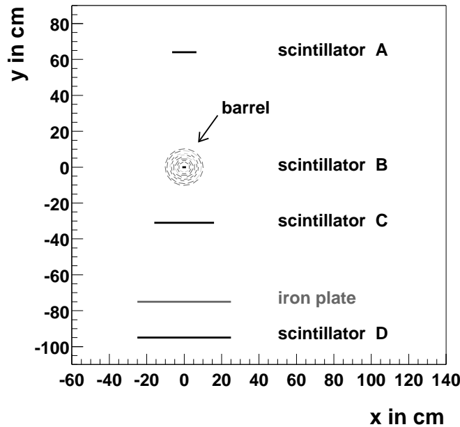
Figure 4.15: Setup for the cosmic ray test (to scale).
