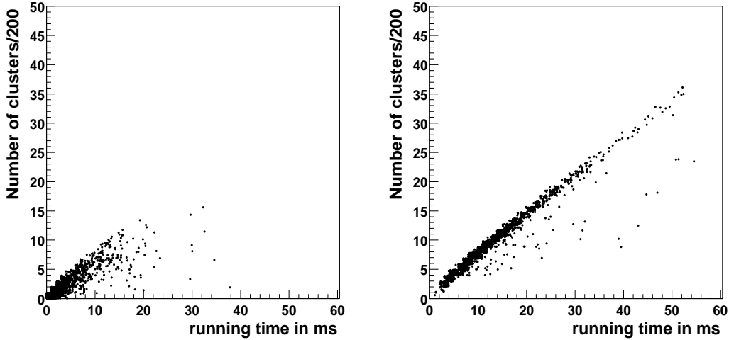
(a) Timing results for Z \rightarrow \mu\mu events without any minimum bias events added.
