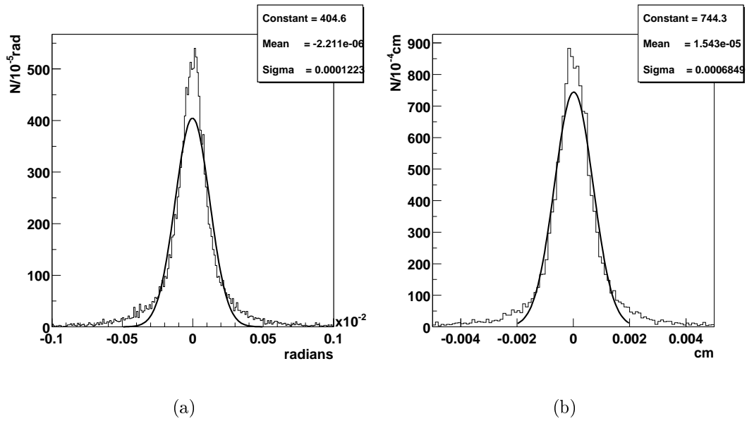
Figure 4.5: Spatial resolution for the barrels: (a) difference in the angle \phi between reconstructed and MC clusters, (b) resolution in x_{\text{local}} ( \Delta(x_{\text{local}}^{\text{reco}} - x_{\text{local}}^{\text{MC}}) ). The fitted function is a Gaussian.
