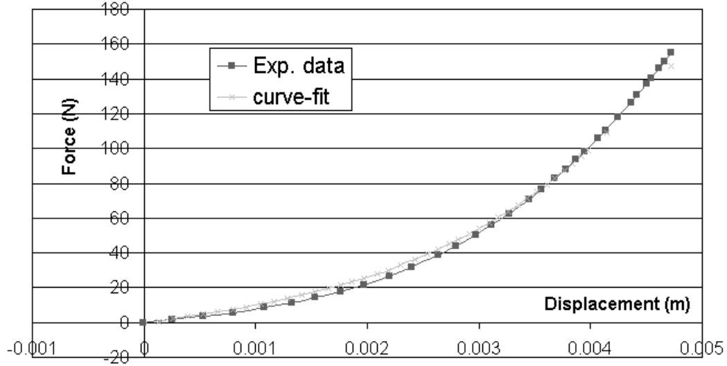
Figure C.8: Static test
