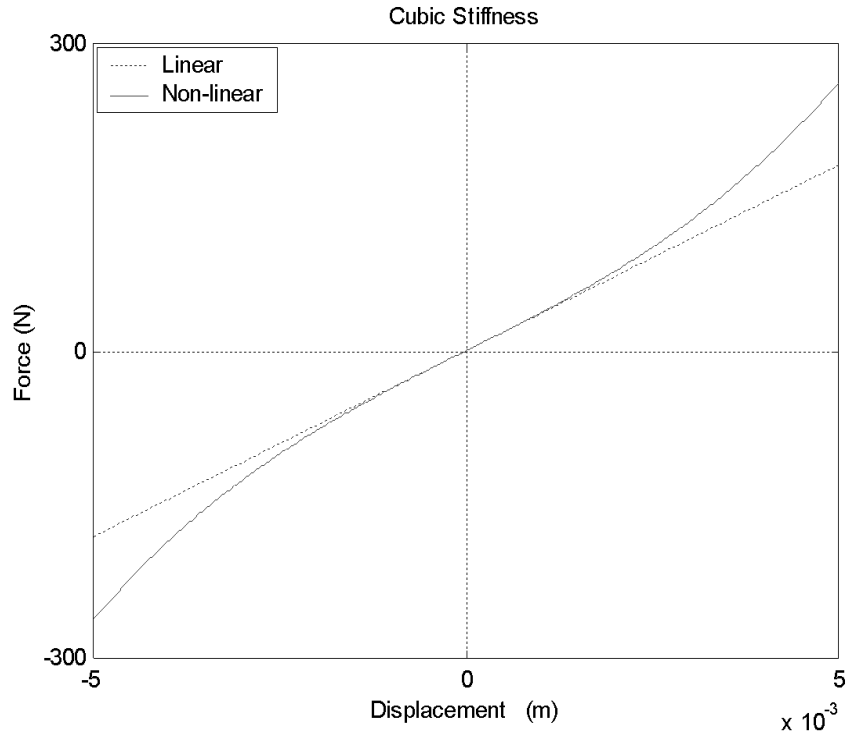
Figure 3.1: Behaviour of a cubic stiffness element
