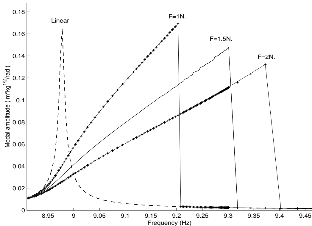
Figure 8.14: HBM results for the first modal amplitude, for three different excitation levels, F = 1N , F = 1.5N and F = 2N (solid line). Also shown in “+” marks, are the polynomial-based predictions
