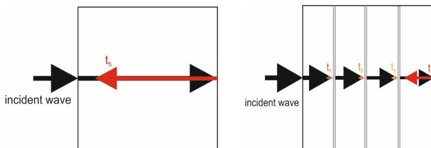
Figure 2: Schematic of reflected wave from a monolithic ceramic (left) and from impedance engineered composite with interfaces with small impedance mismatches.
