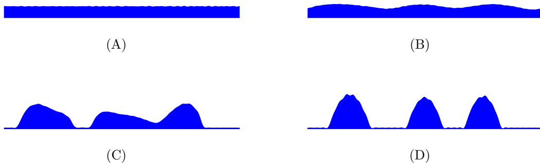
Fig. 6 Temporal evolution of the thin film under the influence of the disjoining potential, \phi(h) = \frac{h^{-3}}{30} - \frac{h^{-2}}{2} for \sqrt{2T} = 0.01 and l_x = 0 . The sequence is organised in time as follows (A)→(B)→(C)→(D).
