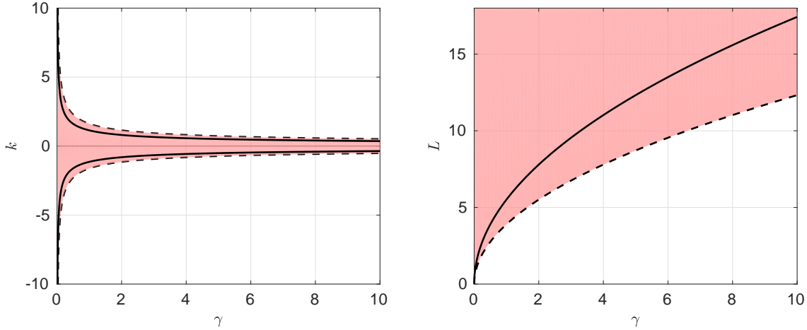
Fig. 2 Linear stability of the uniform state for the interaction potential \phi = \alpha h^{-3} - \beta h^{-2} with \alpha = \frac{1}{30} and \beta = \frac{1}{2} as a function of the surface tension coefficient, \gamma . Panel (a) shows the stability map in terms of the k and \gamma values, whereas panel (b) shows the same on the L - \gamma plane. Shaded red regions correspond to the parameter values for which the system is unstable. Dashed lines represent the critical stability curve given by Eq. (31b) and (32). Solid lines represent the values associated with the maximum growth rate, Eq. (33).
