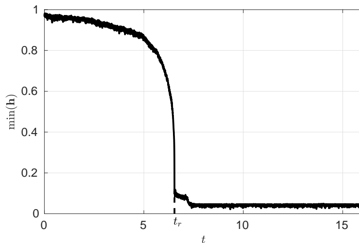
Fig. 7 Single-path variation of the minimum film height near the rupture time with \sqrt{2T} = 0.01 and l_x = 0 .
