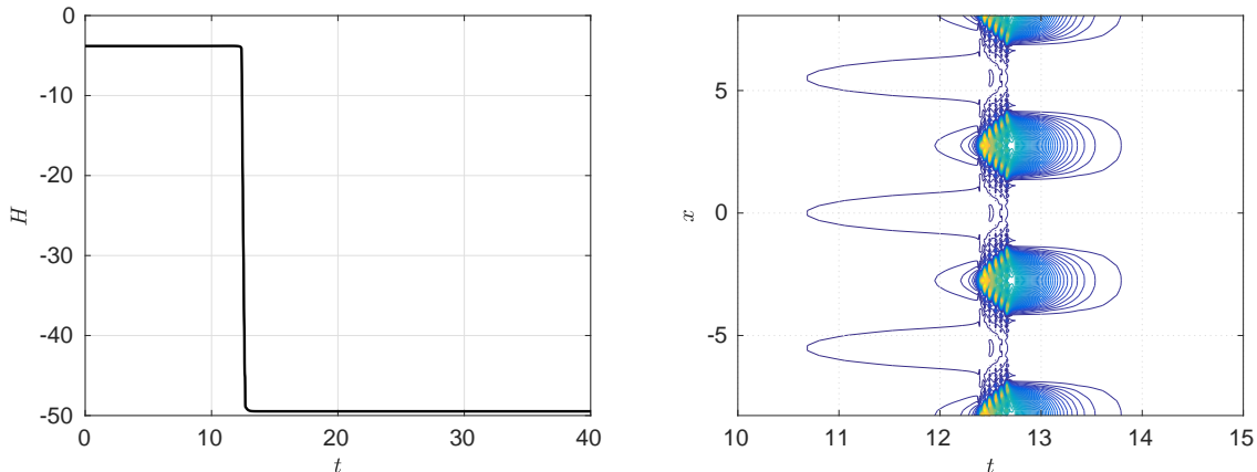
Fig. 5 Evolution of the energy functional \mathcal{H} as a function of time (left), showing two minima: the uniform and droplet states, and of its functional derivative \frac{\delta \mathcal{H}}{\delta h} near the rupture time (right), where the two white regions represent values of x and t for which the functional derivative is zero.
