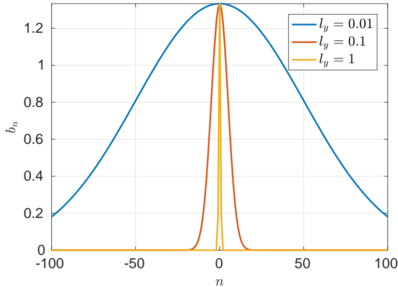
Fig. 3 Distribution of the eigenvalues b_n of the covariance operator Q for different values of the correlation length along the wall-normal direction.
