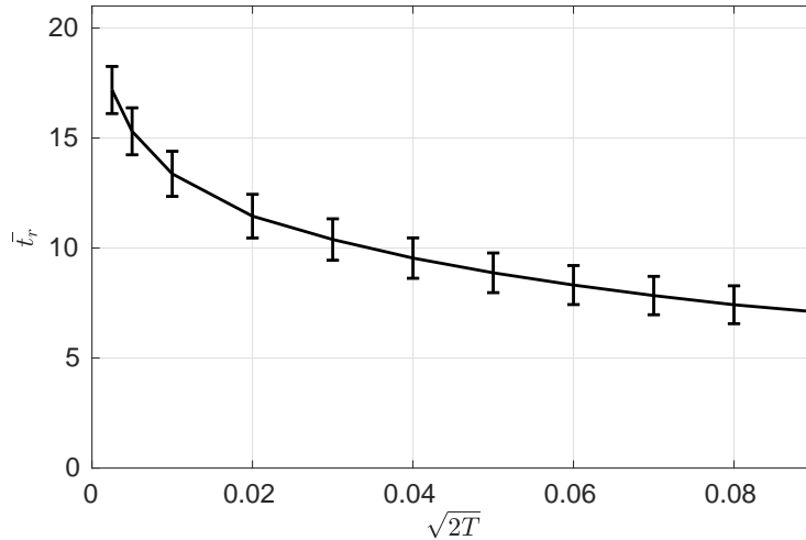
Fig. 8 Mean rupture time \bar{t}_r as a function of the noise intensity \sqrt{2T} . Error bars show the standard deviation of \bar{t}_r .
