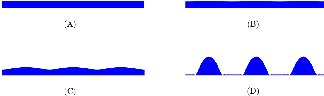
Fig. 4 Deterministic evolution of a thin film under the influence of the disjoining potential, \phi(h) = \frac{h^{-3}}{30} - \frac{h^{-2}}{2} . The sequence must be understood in the following order (A)→(B)→(C)→(D). The uniform solution destabilises and then converges to a second stationary solution which has a cluster-like structure, i.e. the film ruptures and breaks up into droplets.
