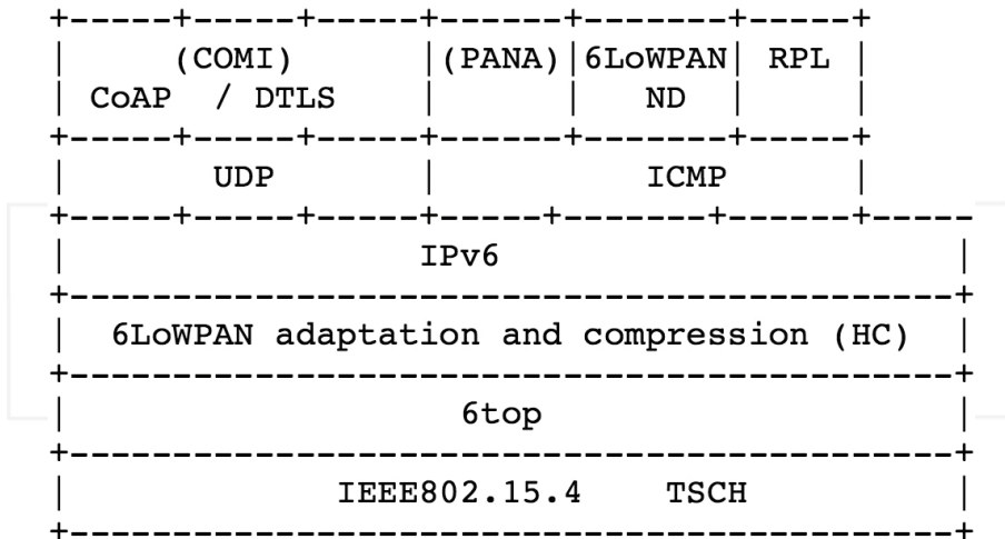
Figure 1. The 6TiSCH Protocol Stack [84].
