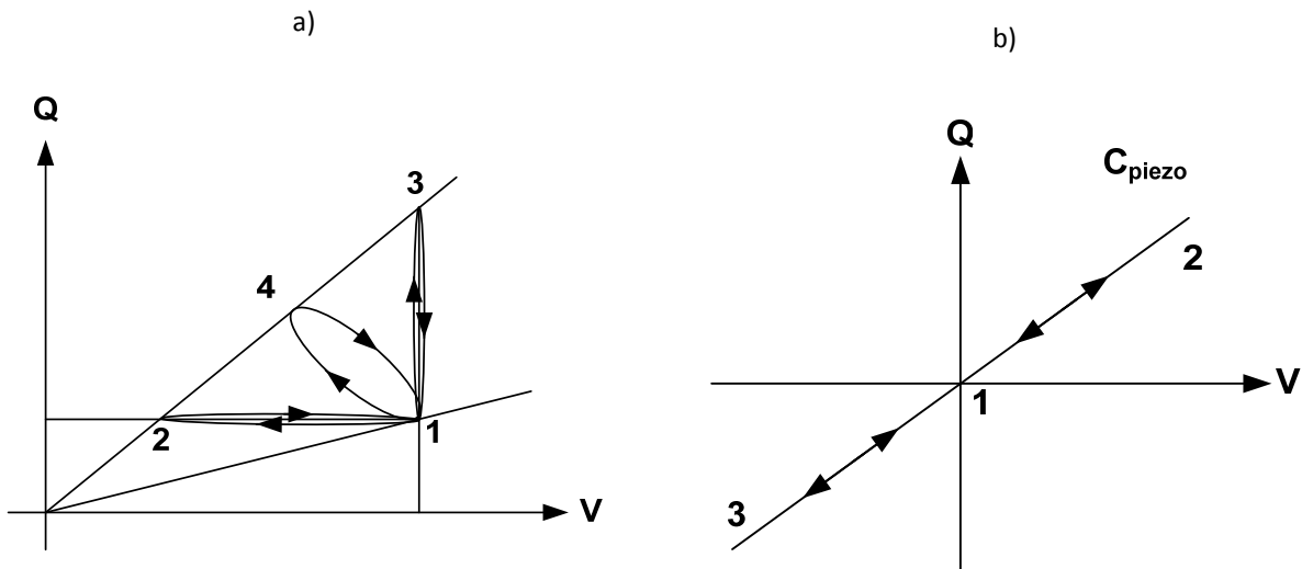
Figure 4 Operation of an electrostatic generator in continuous mode (a) or using a piezoelectric polarisation (b)
