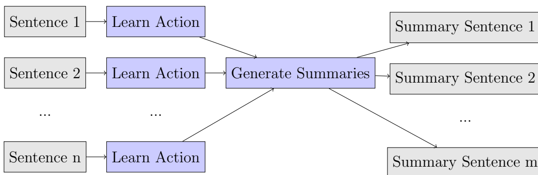
Figure 4.1: ASG steps
