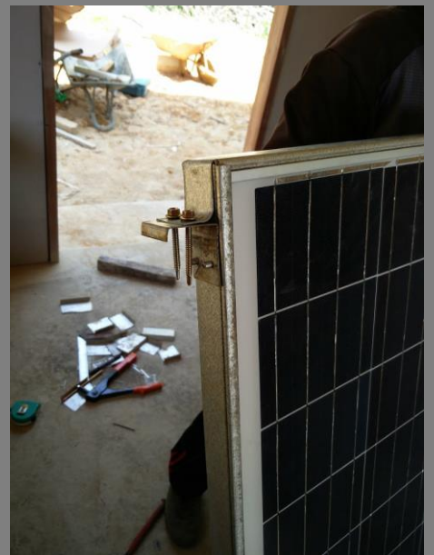
Figure 36: Housing lock.
